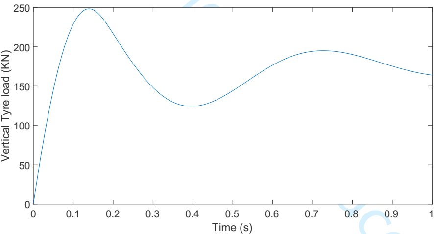
Fig. 5 Variations of the vertical ground force versus time.
