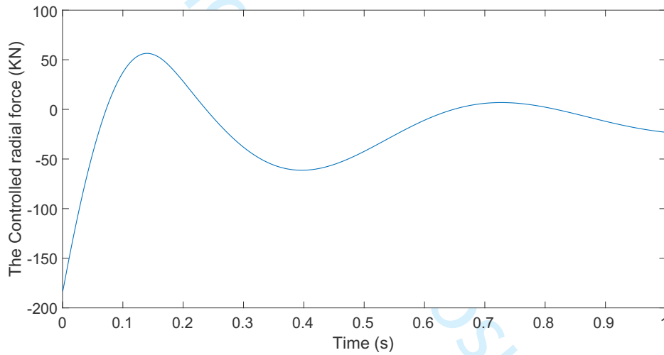
Fig.6 Desired radial force should be replicated by the proposed setup.
