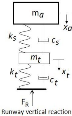
Fig. 3 Vertical suspension model of the aircraft.
