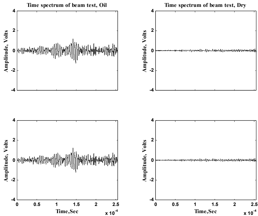
Figure 6 (c – d): Typical stress waves signatures for steel beam tests
