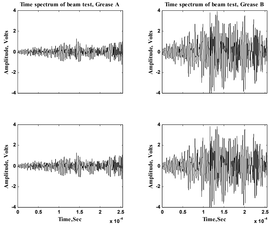
Figure 6 (a – b): Typical stress waves signatures for steel beam tests
