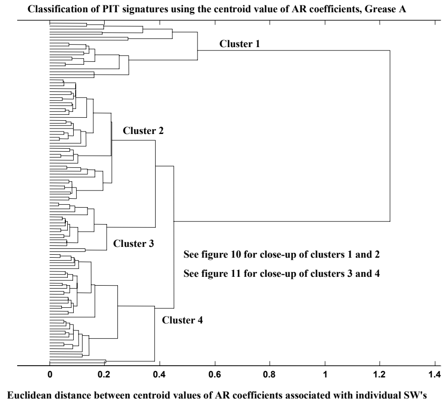
Figure 9: Classification of all filling capacity, oil lubrication and dry condition signatures based on AR technique, grease A.
