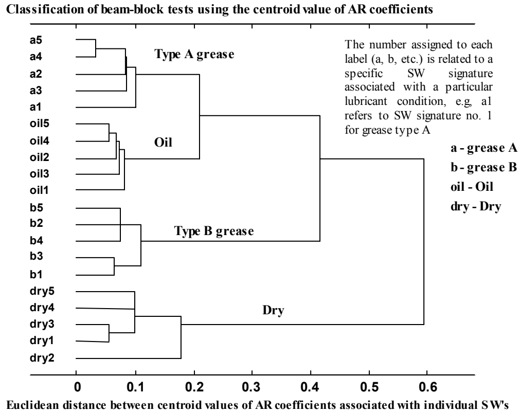
Figure 7: Classification of the PIT signatures based on the AR coefficients, steel blocks test
