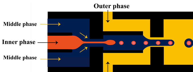
Figure 5. Two consecutive flow-focusing drop generators with different wettability for producing core/shell drops. The upstream and downstream orifice was wetted with the middle and outer fluid, respectively [111].
