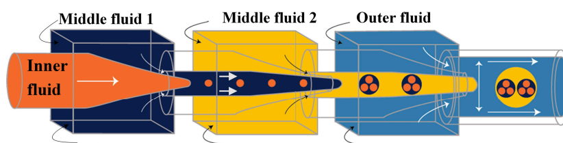
Figure 24. Generation of quintuple-component triple emulsions in a microfluidic device consisted of three co-flow drop makers [54].
