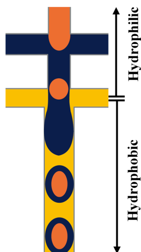
Figure 8. A poly(dimethylsiloxane) (PDMS) device with two serial cross junctions for formation of O/W/O double emulsion using two consecutive emulsification steps. The dripping instabilities are present in both junctions; the inner phase is emulsified at the first junction followed by the middle phase at the second junction [109].
