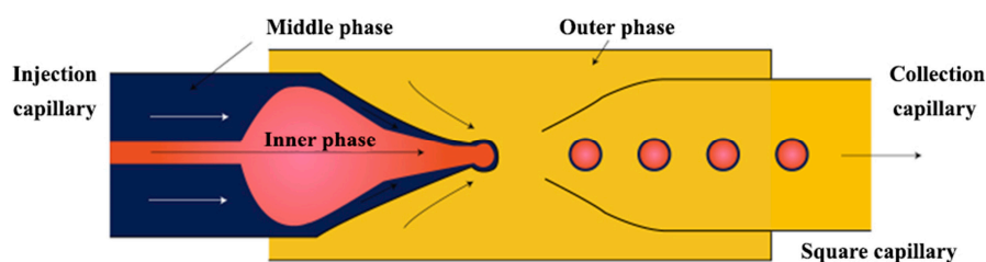
Figure 16. Glass capillary device for the formation of thin shelled drops. The middle phase has a higher affinity towards the wall of the outer injection capillary and flows in a thin layer along the wall of the outer capillary pushed by the inner phase injected at high flow rate through the innermost capillary [31].
