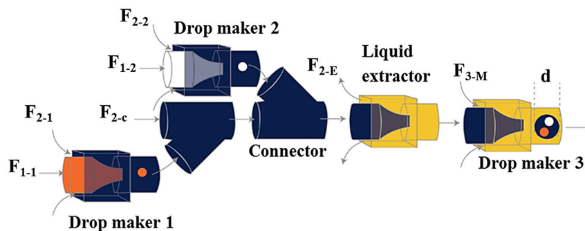
Figure 20. Generation of quadruple-component double emulsions using an assembly consisted of 3 drop makers, 2 connectors, and one liquid extractor. A PVC tube is used to connect the round capillaries of two adjacent drop makers. F_{i-j} is the inlet/outlet stream at each level, where the subscripts i and j refer to the level number and the injection position respectively. The drop maker 1 generates the inner drops of F_{1-1} , the drop maker 2 generates the inner drops of F_{1-2} , and the drop maker 3 generates the outer drops of F_{3-M} [61].
