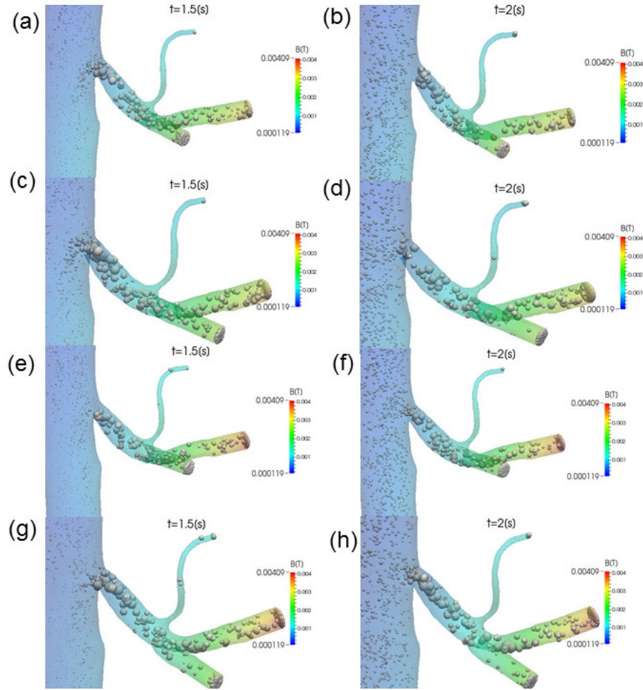
Figure 7: Magnetic Induction Field and particle positions at different time steps, for the different conditions listed in Table 1. (a) 1st run t = 1.5\text{s} ; (b) 1st run t = 2\text{s} ; (c) 2nd run t=1.5\text{s} ; (d) 2nd run t= 2\text{s} ; (e) 3rd run t = 1.5\text{s} ; (f) 3rd run t = 2\text{s} ; (g) 4th run t=1.5\text{s} ; (h) 4th run t= 2\text{s} .
