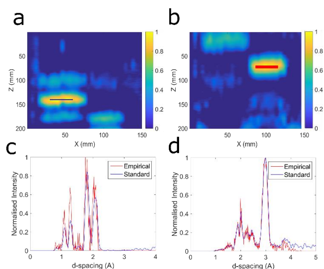
Fig 2. Match coefficients mapped onto the (Z,X) plane are created by comparing empirical diffractograms against a copper (a) and calcite (b) standard. The true locations of the copper and calcite samples are illustrated by the blue and red boxes, respectively. Example diffractograms illustrating good match coefficients are also illustrated for copper (c) and calcite (d).
