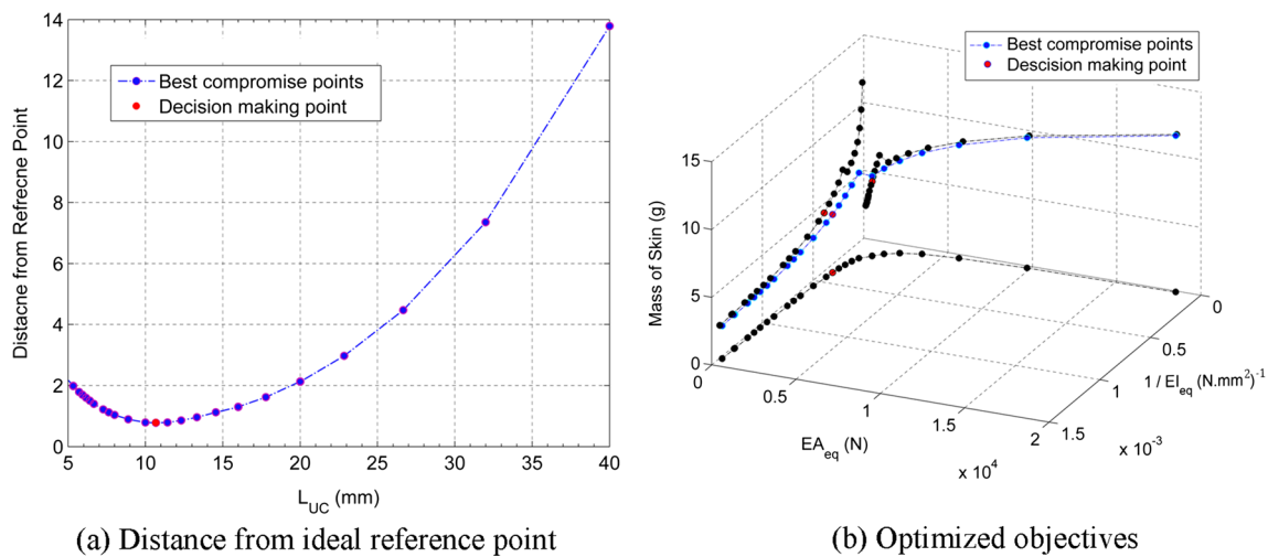
Fig. 14 Entire best compromise points for different length of unit cells
