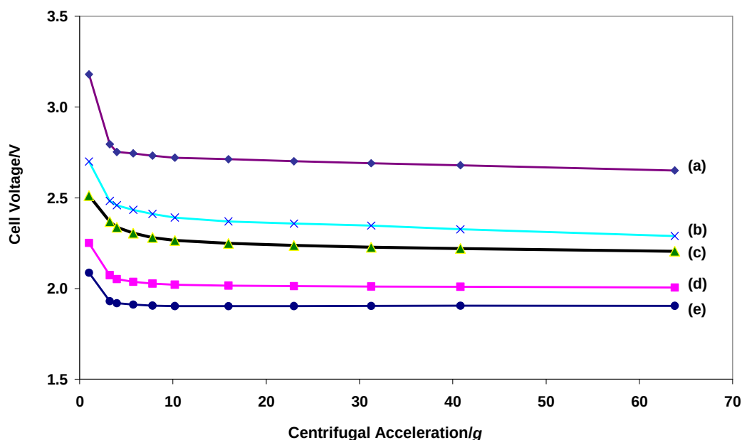
Figure 10 Cell voltage against centrifugal acceleration (in g ) for the rotary cell at different current densities, with electrodes made of nickel mesh upon stainless steel plate. Different curves were corresponding to data from different current densities of (a) 22.5 \text{ kA m}^{-2} , (b) 13.5 \text{ kA m}^{-2} , (c) 9.0 \text{ kA m}^{-2} , (d) 4.5 \text{ kA m}^{-2} and (e) 2.3 \text{ kA m}^{-2} . 7.7 M KOH solution was used; solution bulk temperature, 344 K.
