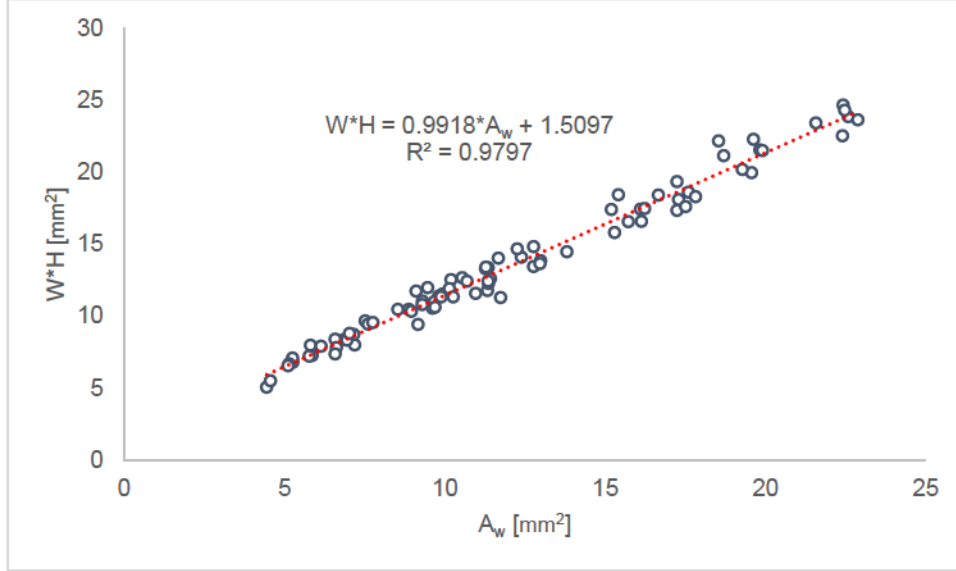
Fig. 2. Relationship between the cross-section area ( A_w ) and the product between layer height ( H ) and wall width ( W )
