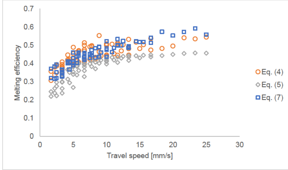
Fig. 6. Melting efficiency as a function of travel speed for the cold metal transfer process
