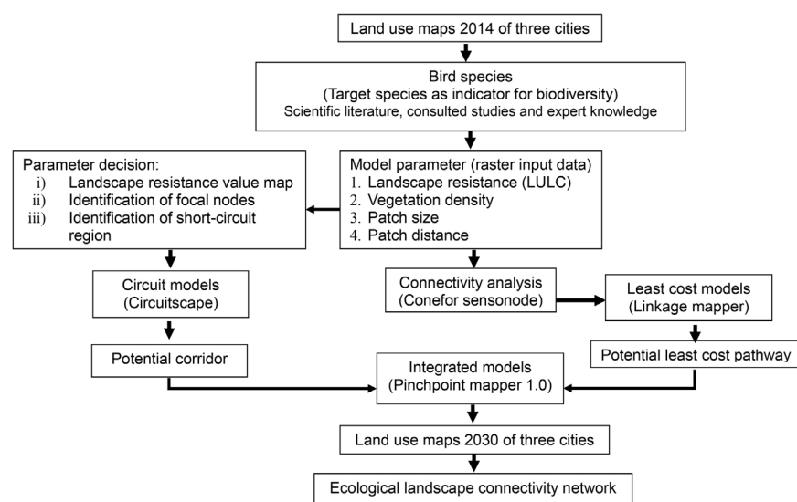
Fig. 2. Methodological framework.
