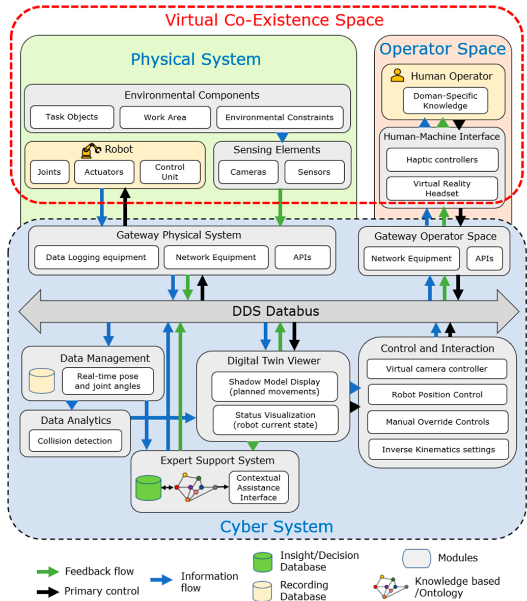
Figure 1. The system architecture of the proposed VR-based teleoperation system.
