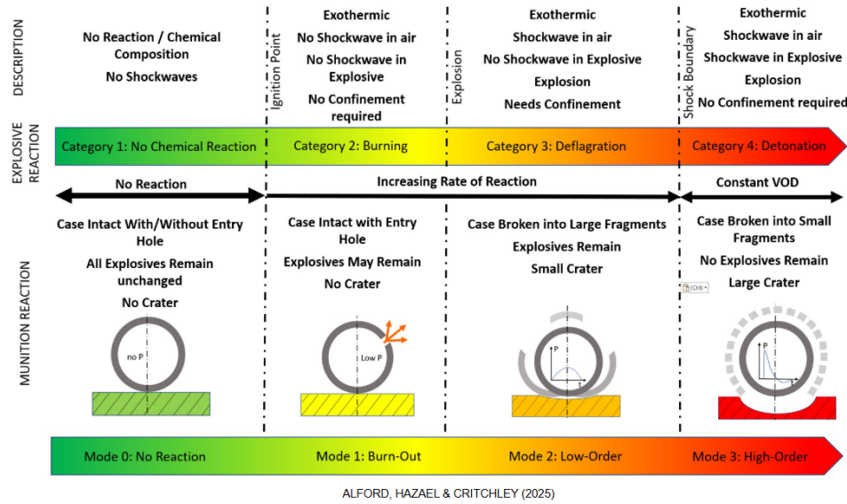
Figure 1: Combined Combustion 12 Continuum & EOD Munition Reaction Scale
