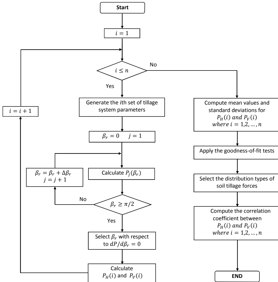
Fig. 3 – Flow chart of the steps involved in estimating the variability of tillage forces based on the variability of tillage system parameters
