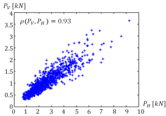
Fig. 9 - Correlation of tillage forces
