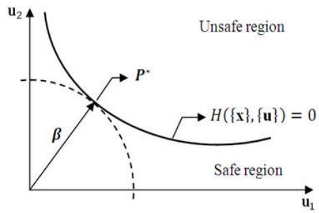
Fig. 5 - The concept of the reliability index in normalized space ( P^* , design point; \beta , reliability index; H(\{x\}, \{u\}) = 0 , limit state function in normalized space)
