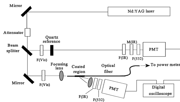
Fig. 5. Schematic diagram of the SHG apparatus: F(vis)'s, visible filters; F(IR)'s, IR filters; F(532)'s, 532-nm bandpass filters; M(IR), IR mirror; PMT's, photomultiplier tubes.
