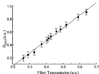
Fig. 7. SHG versus fiber coupled pump power at constant temperature, T = 21.4^\circ\text{C} .
