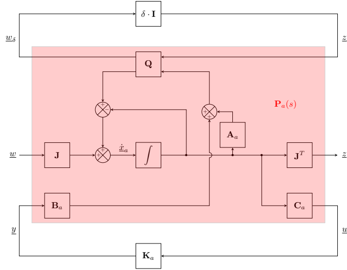
Fig. 2: Block Diagram of Kreiss Constant Re-expression
