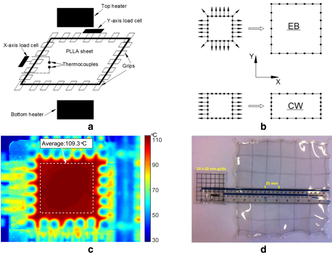
Fig. 4 Biaxial stretch testing, (a) machine arrangement; (b) deformation mode (EB: equal biaxial, CW: constant-width); (c) thermal images of a testing sample at 110^\circ\text{C} [38]; (d) a testing sample marked with grid lines before and after stretch [38]
