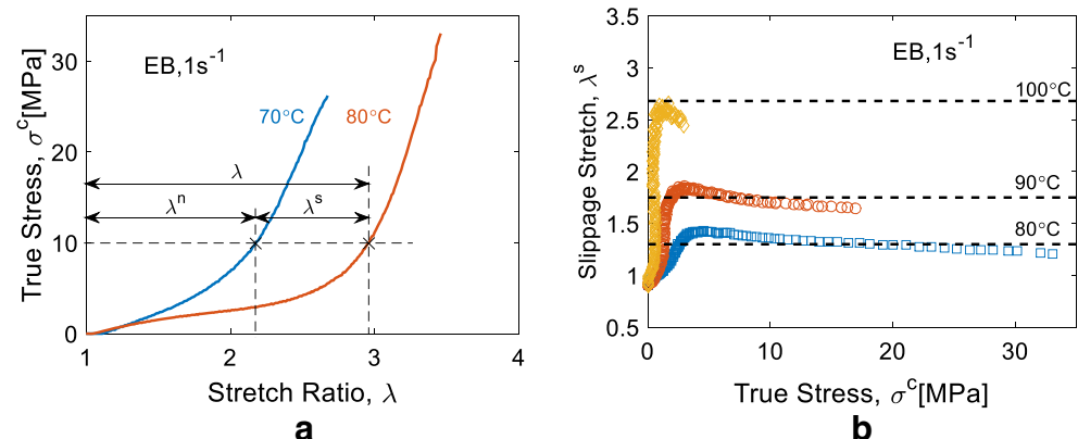
Fig. 15 Slippage effect for conformational component (a) split of total stretch; (b) slippage stretch at EB deformation
