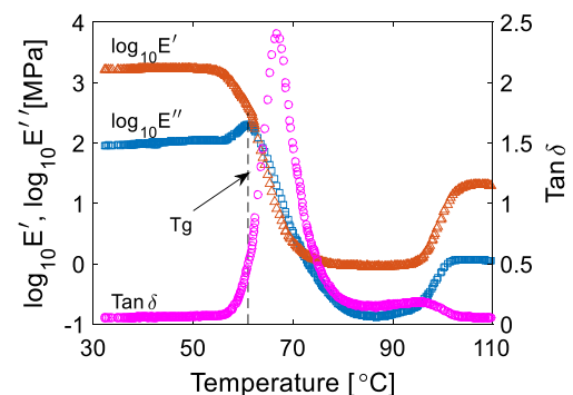
Fig. 3 DMA results of extruded PLLA sheets
