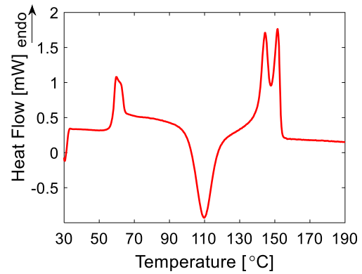
Fig. 2 DSC thermal curve of extruded PLLA sheet
