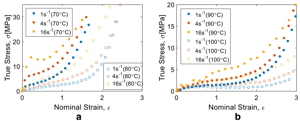
Fig. 8 Influence of strain rate on the stress-strain behaviour of PLLA sheets under EB deformation (a) at temperatures 70 °C and 80 °C, and (b) at temperatures 90 °C and 100 °C
