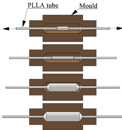
Fig. 1 Stretch blow moulding of PLLA tubes
