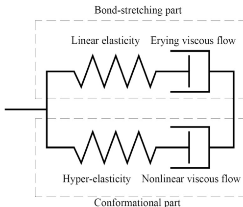
Fig. 5 One dimensional representation of glass-rubber (GR) model
