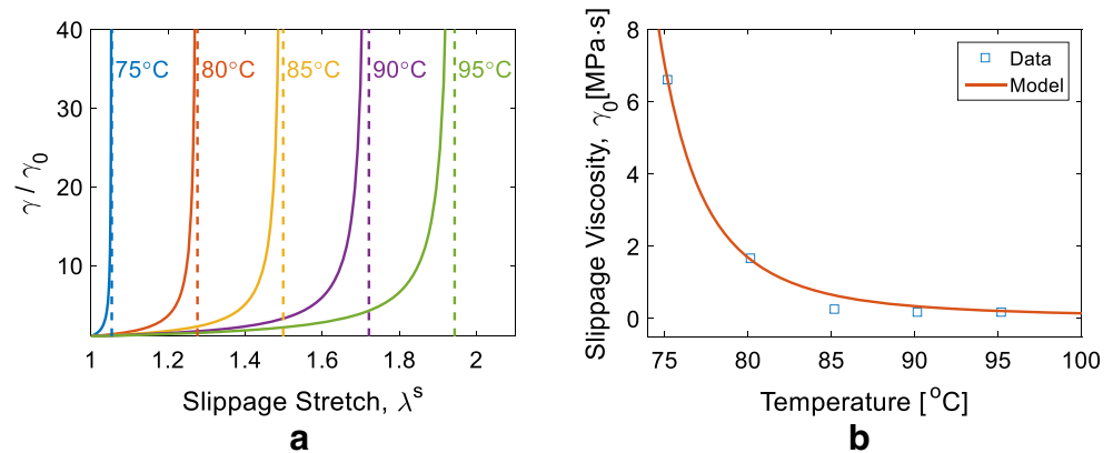
Fig. 16 Slippage viscosity properties, (a) evolution of slippage viscosity; (b) initial slippage viscosity at different temperatures and strain rate of 1 \text{ s}^{-1}
