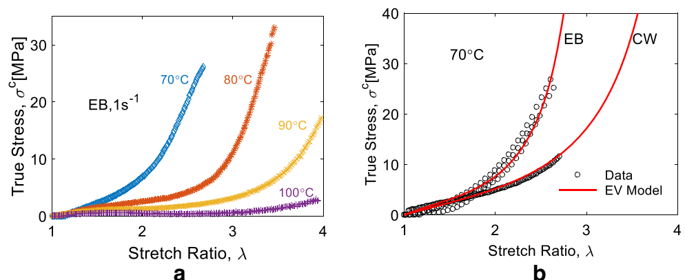
Fig. 13 Conformational component, (a) conformational stress; (b) curve fitting for EV model
