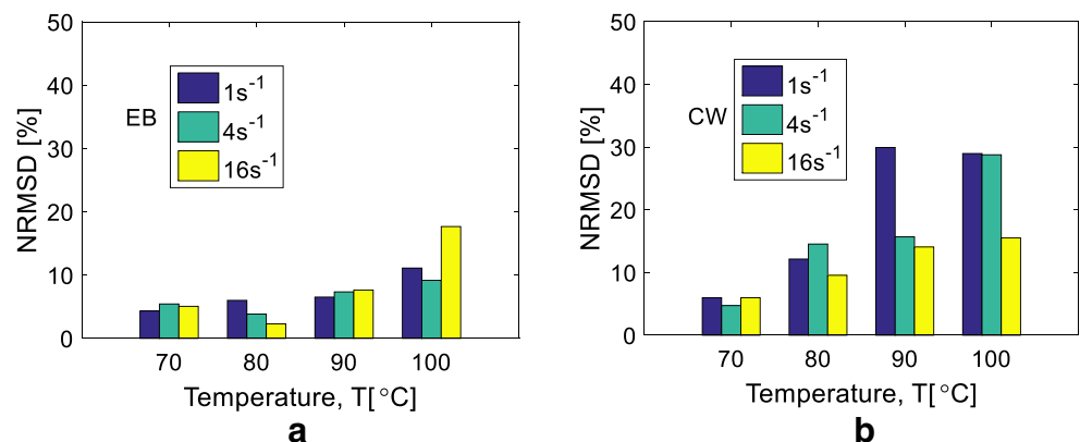
Fig. 18 Normalized root mean square deviation between results from simulation and experiments at two deformation modes, (a) EB; (b) CW
