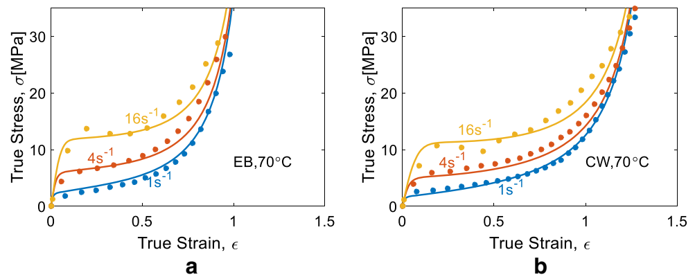
Fig. 14 Comparison of stress-strain relations at temperature of 70 °C (lines: modelling, markers: experiment), (a) at EB deformation; (b) at CW deformation
