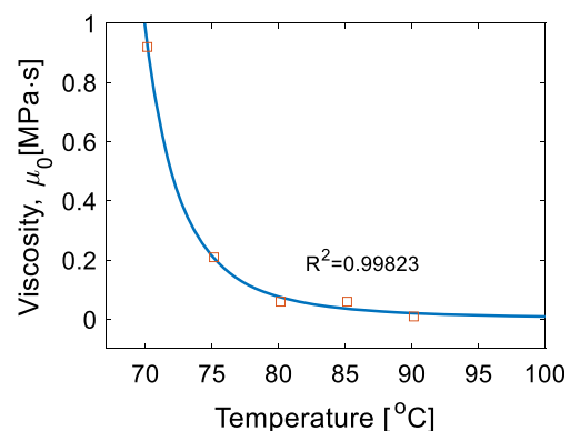
Fig. 11 Bond-stretching viscosity with temperature
