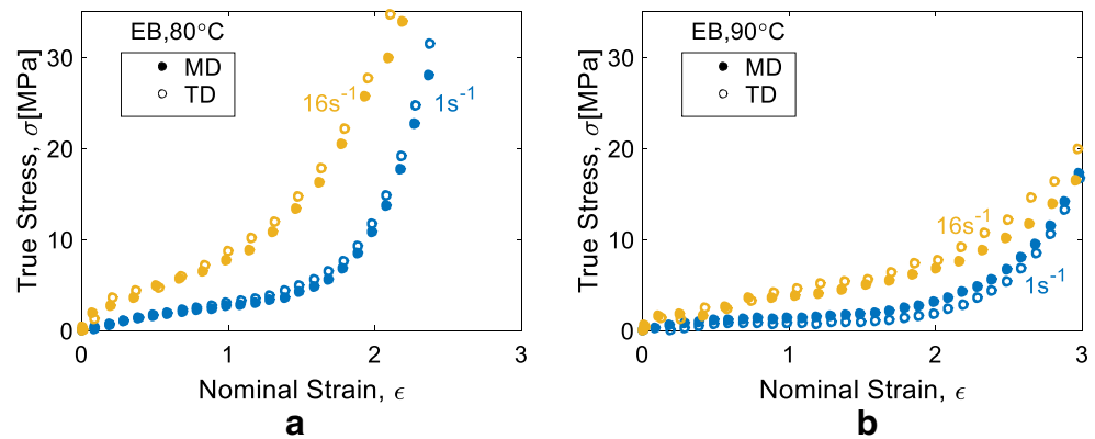
Fig. 6 Comparison of stress strain curves from MD and TD directions of PLLA sheets (a) at 80 °C, (b) at 90 °C
