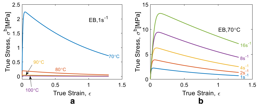
Fig. 12 Bond-stretching stress by GR model, (a) temperature effect; (b) strain rate effect
