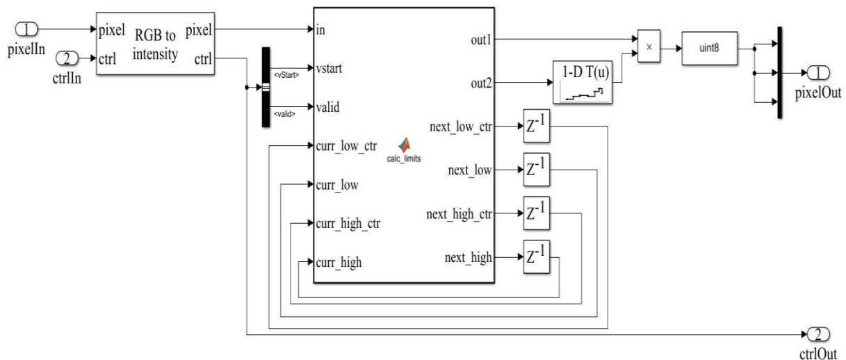
Fig. 3. Internal circuitry of 'ContrastStretch_HW' module.
