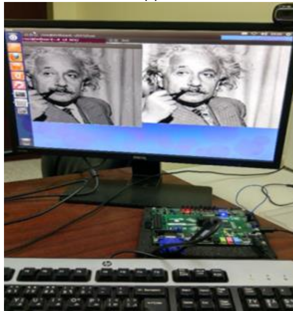
Fig. 5. HW-SW co-design: a) block diagram; b) implementation on Zedboard to test the developed contrast stretching IP core.
