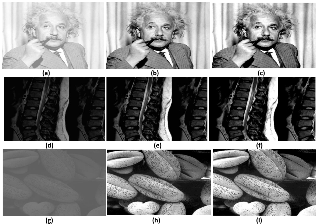
Fig. 9. Comparison of hardware and software models output on test images: a, d, g) input images; b, e, h) processed through Software; c, f, i) processed through hardware leading to average(max.) error per pixel values of 1.075(4), 1.4(4) and 3.1(10), respectively on the tested images.
