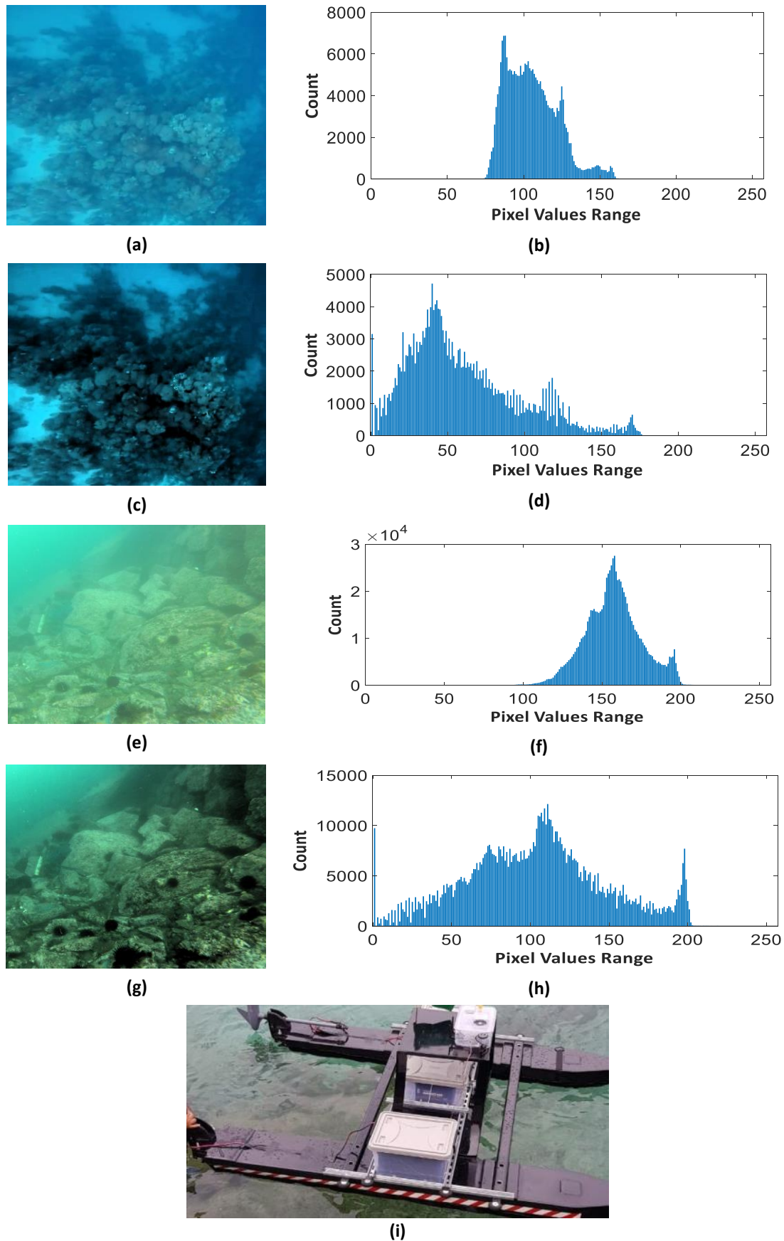
Fig. 10. Visual results of contrast enhancement of underwater video frames using the proposed online algorithm: a) input frame 1; b) input frame 1 histogram; c) processed frame 1; d) processed frame 1 histogram; e) input frame 2; f) input frame 2 histogram; g) processed frame 2; h) processed frame 2 histogram; i) underwater video capturing system on-board explorer boat.
