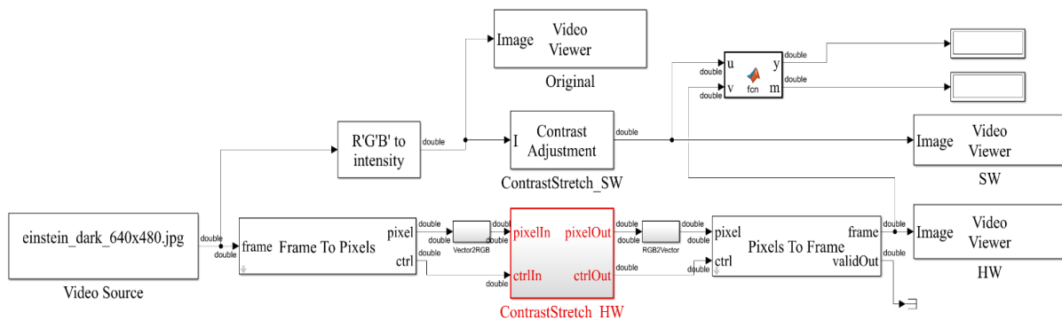
Fig. 2. Top-level Simulink model for development and testing of the proposed hardware for contrast stretching algorithm with adaptive limits.
