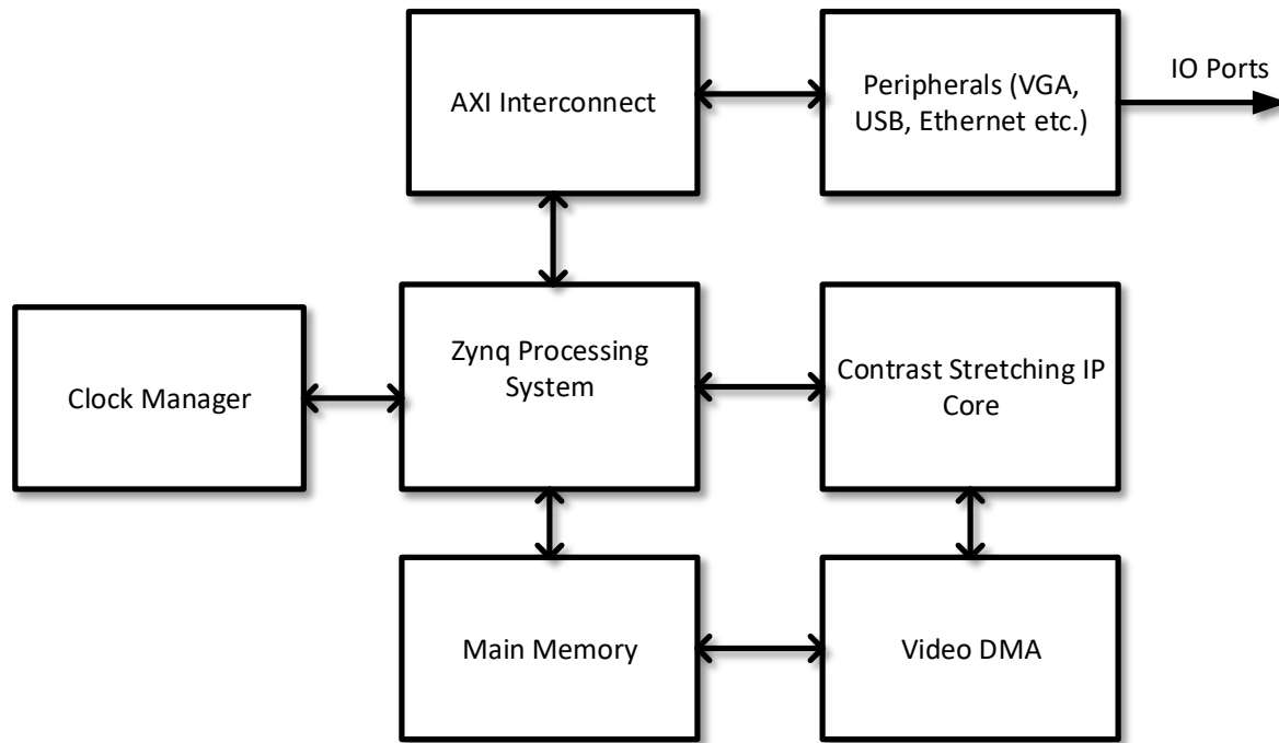
Fig. 6. HW-SW co-design components' integration in the Vivado project.
