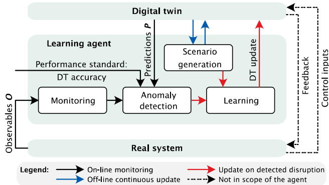
Fig. 1: Architecture of the learning agent.
