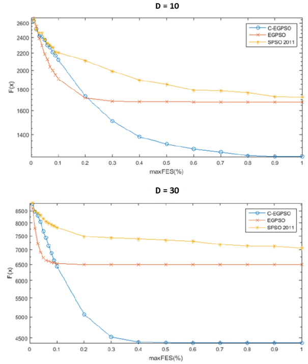
Fig. 7. Comparison of the convergence of the best value for problem F_4 of CEC2015 benchmark in dimension D = 10 (top) and dimension D = 30 (bottom).
