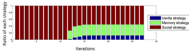
Fig. 5. Evolution of the strategies over the time for one randomly chosen particle. This example shows the ratio of each strategy over the time for a simple sphere problem.
