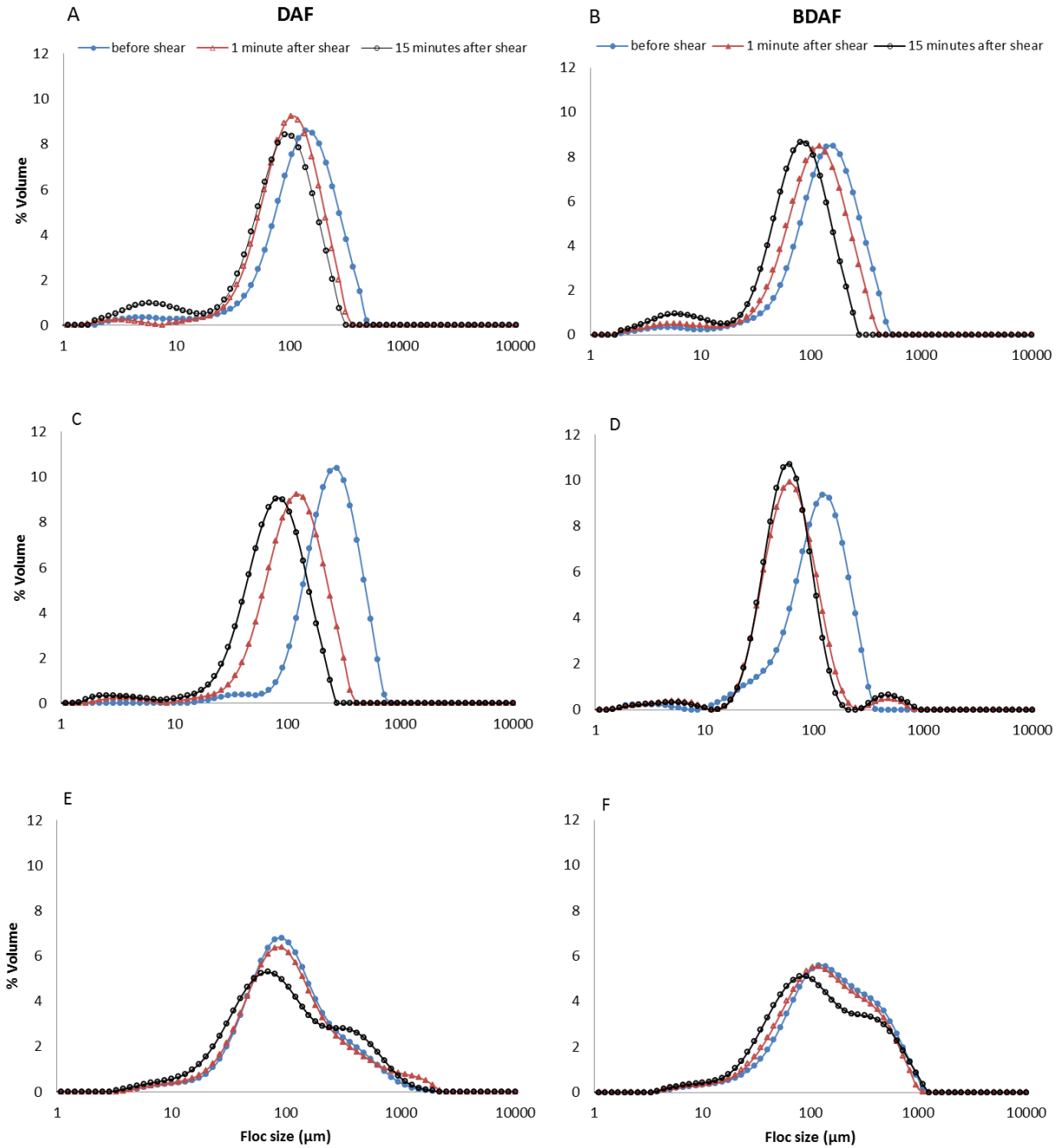
Figure 4 Floc breakage profile for DAF (left column) and BDAF (right column) system, of S. obliquus (A and B), C. vulgaris (C and D) and A. maxima (E and F), before and after exposure to a shear rate of 200 rpm.
