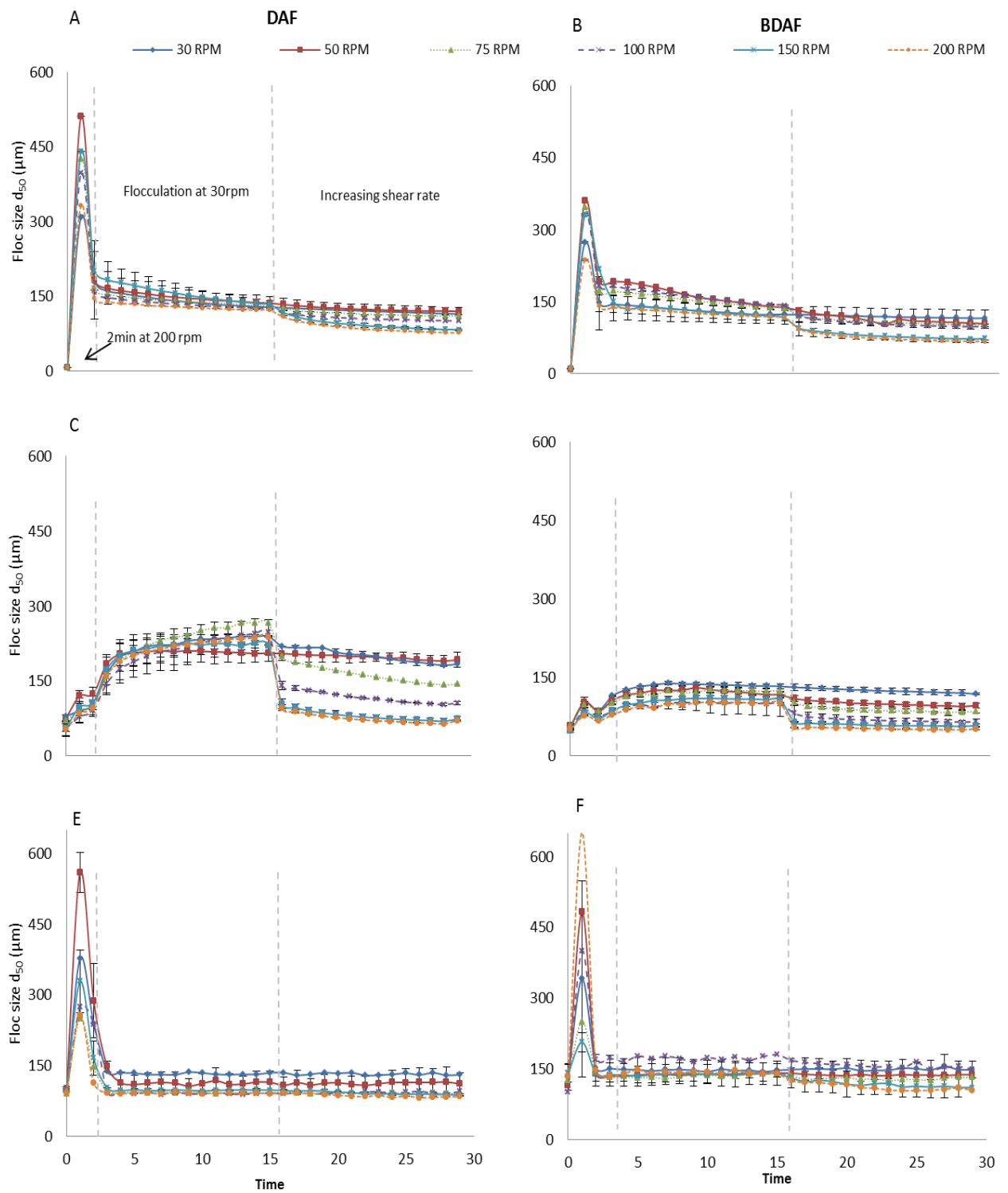
Figure A.1 Floc growth and breakage profile for DAF (left column) and BDAF (right column) system, of S. obliquus (A and B), C. vulgaris (C and D) and A. maxima (E and F) at increasing shear rate (on support of paragraph 3.1)
