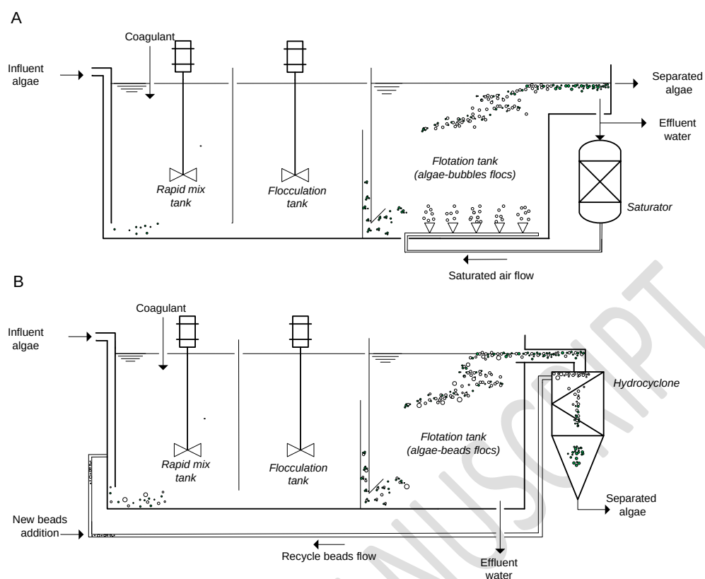
Figure 1 Schematic representation of Dissolved Air Flotation (A) and Ballasted Dissolved Air Flotation (B) systems.
