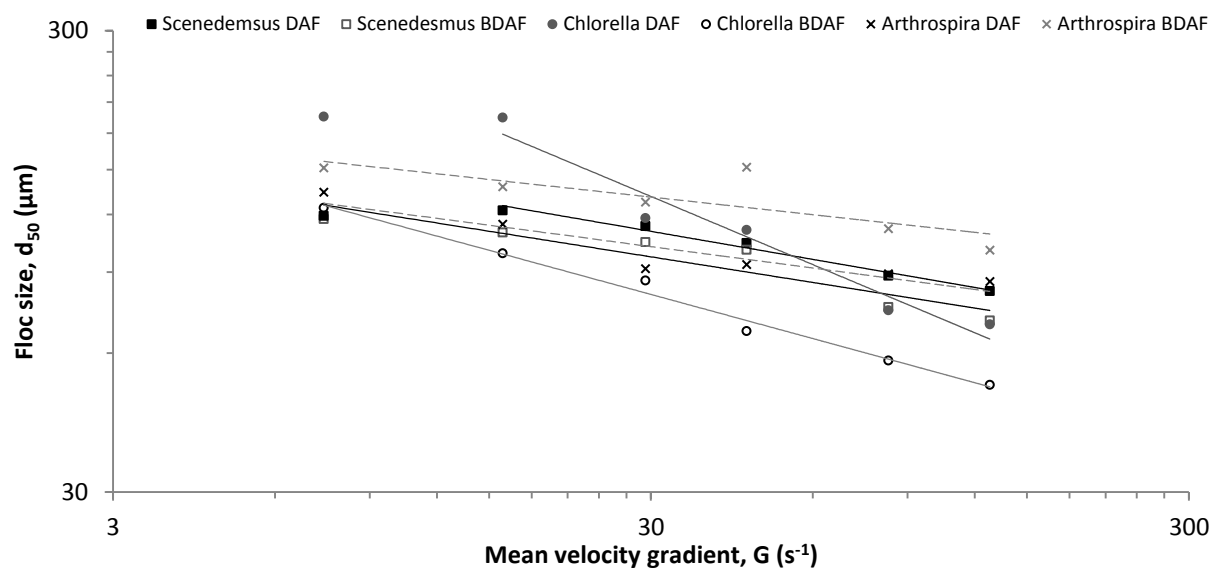
Figure 3 Log log plot of steady state floc size vs increasing shear rate plotted as G , with and without microspheres addition.
