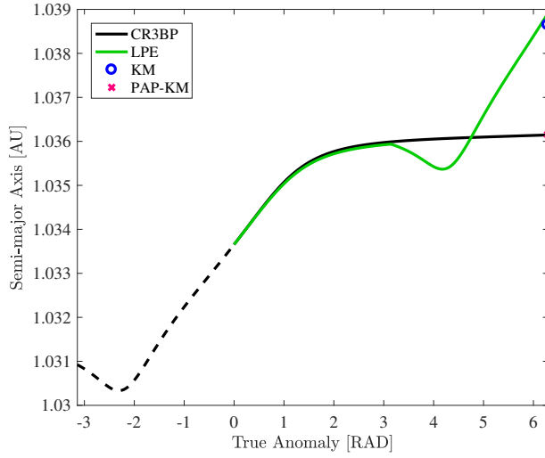
Fig. 4: Semi-major axis evolution of one orbital period for asteroid 2018 AV2. Extra back-propagation of half a period for the CR3BP in a dashed line
