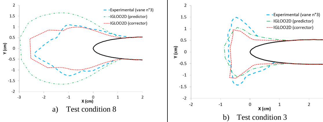
Fig. 19 Numerical results for ice accretion on vanes (predictor and corrector approach)
