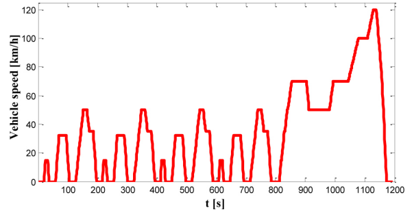
Figure 1. Road test under the NEDCE driving cycle.
