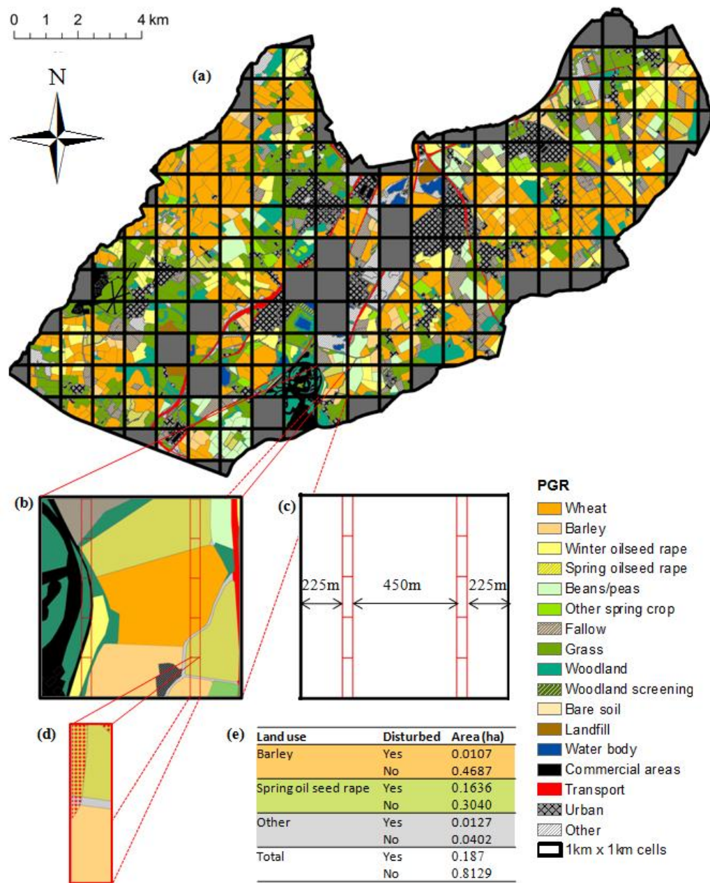
Fig. 2. The different steps run within BirdMod to quantify habitat availability prior to reclassification into functional space: (a) location of the 1 km x 1 km squares within the Marston Vale, (b) example of the location of the 200 m x 50 m transect sections (red lines) within each square, (c) distance between parallel transects, (d) detail of the different land uses identified on one of the transects showing the disturbed (red dots) areas and (e) table summarising the land uses for the selected transect as estimated by BirdMod. Grey cells show squares that have been excluded from the analysis (e.g. area of farmland is <50 ha).
