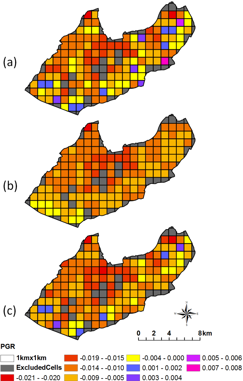
Fig. 3. Mean annual pgr across the 19 bird species predicted for the (a) BASELINE , (b) MAXIMIZE and (c) RESILIENCE scenarios. Positive and negative values were coded using a blue and red coloured scale, respectively. The range and the breaks for each of the scales were determined to enhance visualisation.
