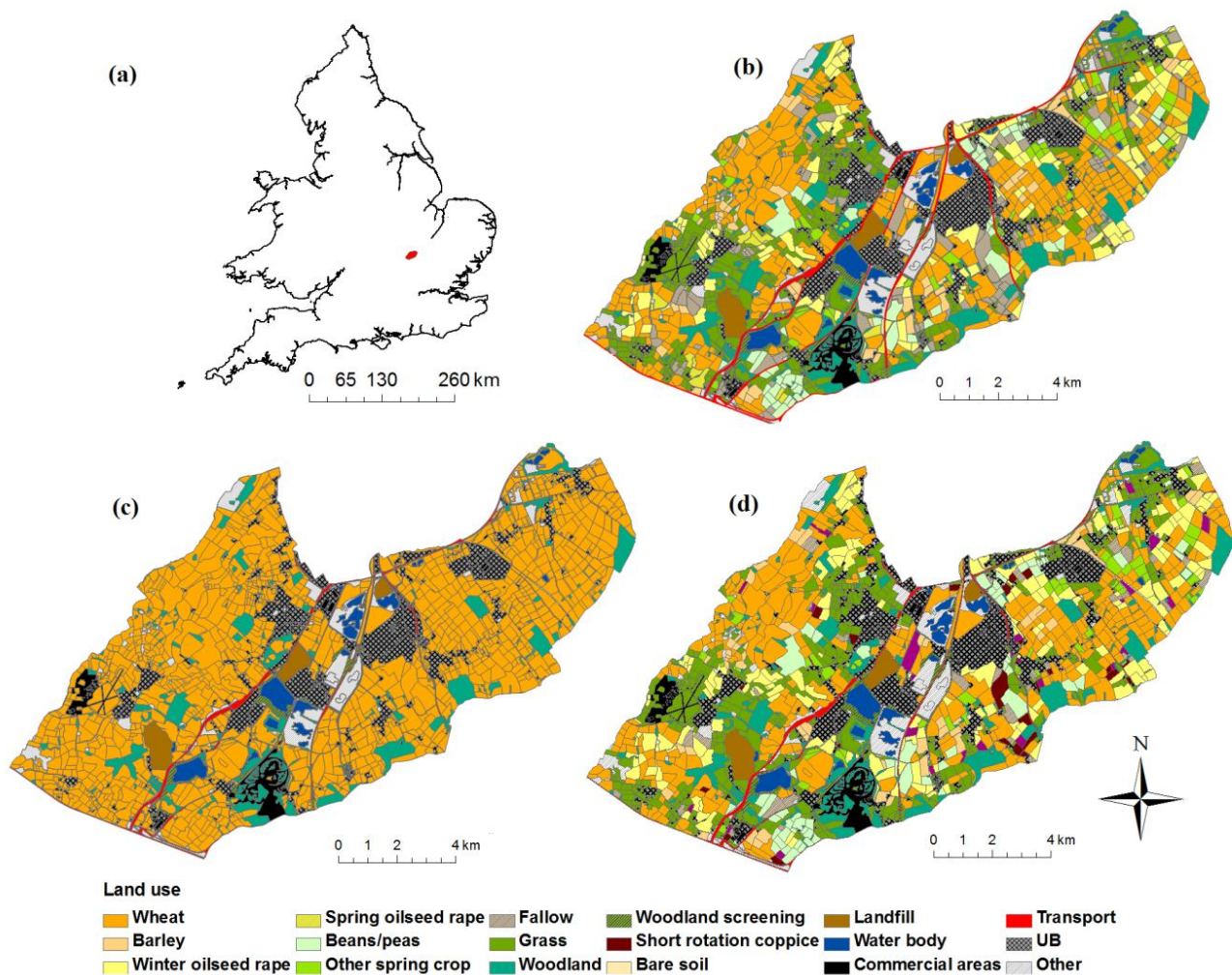
Fig. 1. Land use maps of the Marston Vale (2009): (a) location of the Marston Vale (b) BASELINE , (c) MAXIMIZE and (d) RESILIENCE scenarios.
