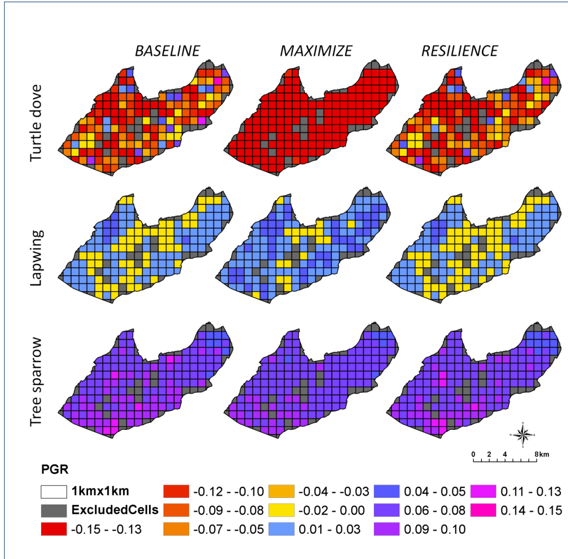
Fig. 4. Spatial variation in predicted annual pgr across Marston Vale for three exemplar species. Positive and negative values were coded using a blue and red coloured scale, respectively. The range and the breaks for each of the scales were determined to enhance visualisation. See Fig. B.2 for equivalent maps for the other 16 species.
