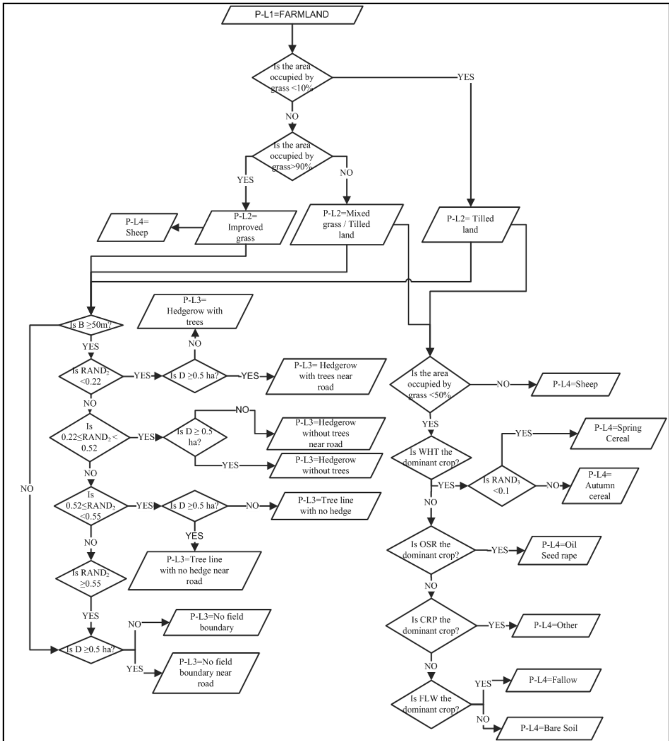
Fig. A.1. Primary habitat allocation algorithm applied when the first tier of classification (P-L1) was FARMLAND. B is the total length of hedges within the 1 km square; D is the total area of disturbed habitat within the transect section; RAND() is a randomly generated number between 0 and 1, with the associated subscript number identifying the tier within the four level hierarchical BBS habitat code structure; P-L1, P-L2, P-L3 and P-L4 represent the four primary habitat levels; and WHT, OSR, CRP and FLW are the land uses coded as specified in Table 1.
