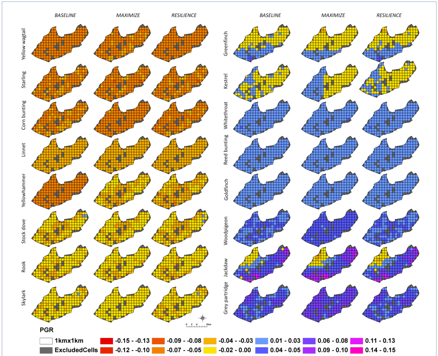
Fig. B.2. Spatial variation in predicted annual pgr across Marston Vale for 16 species not included in Fig. 4. Positive and negative values were coded using a blue and red coloured scale, respectively. The range and the breaks of the scale were determined to enhance visualization.
