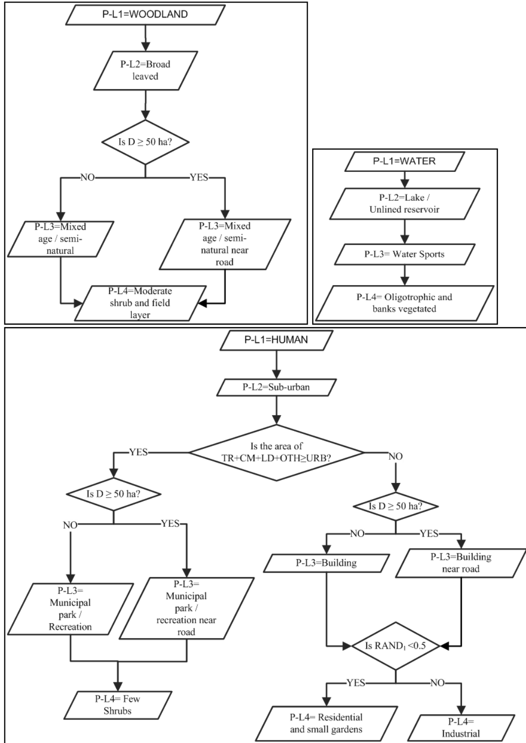
Fig. A.2. Primary habitat allocation algorithm applied when the first tier of classification (P-L1) was WOODLAND, WATER or HUMAN. B is the total length of hedges within the 1 km square; D is the total area of disturbed habitat within the transect section; RAND() is a randomly generated number between 0 and 1, with the associated subscript number identifying the tier within the four level hierarchical BBS habitat code structure; P-L1, P-L2, P-L3 and P-L4 represent the four primary habitat levels; and TR, CM, LD, OTH and URB are the land uses coded as specified in Table 1.
