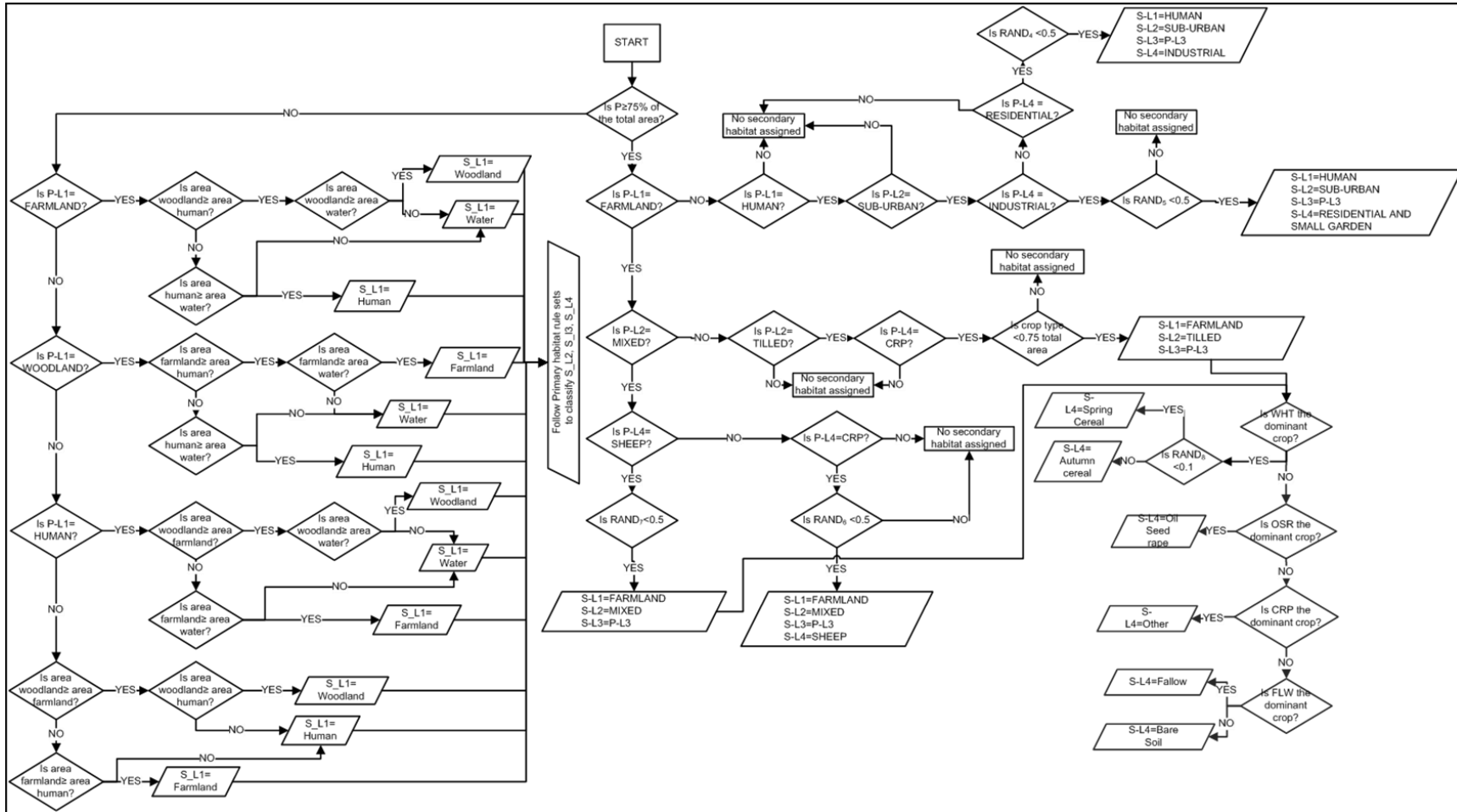
Fig. A.3. Secondary habitat allocation algorithm applied. B is the total length of hedges within the 1 km square; D is the total area of disturbed habitat within the transect section; RAND() is a randomly generated number between 0 and 1, with the associated subscript number identifying the tier within the four level hierarchical BBS habitat code structure; P-L1, P-L2, P-L3 and P-L4 represent the four primary habitat levels; S-L1, S-L2, S-L3 and S-L4 represent the four secondary habitat levels; and WHT, OSR, CRP and FLW are the land uses coded as specified in Table 1.
