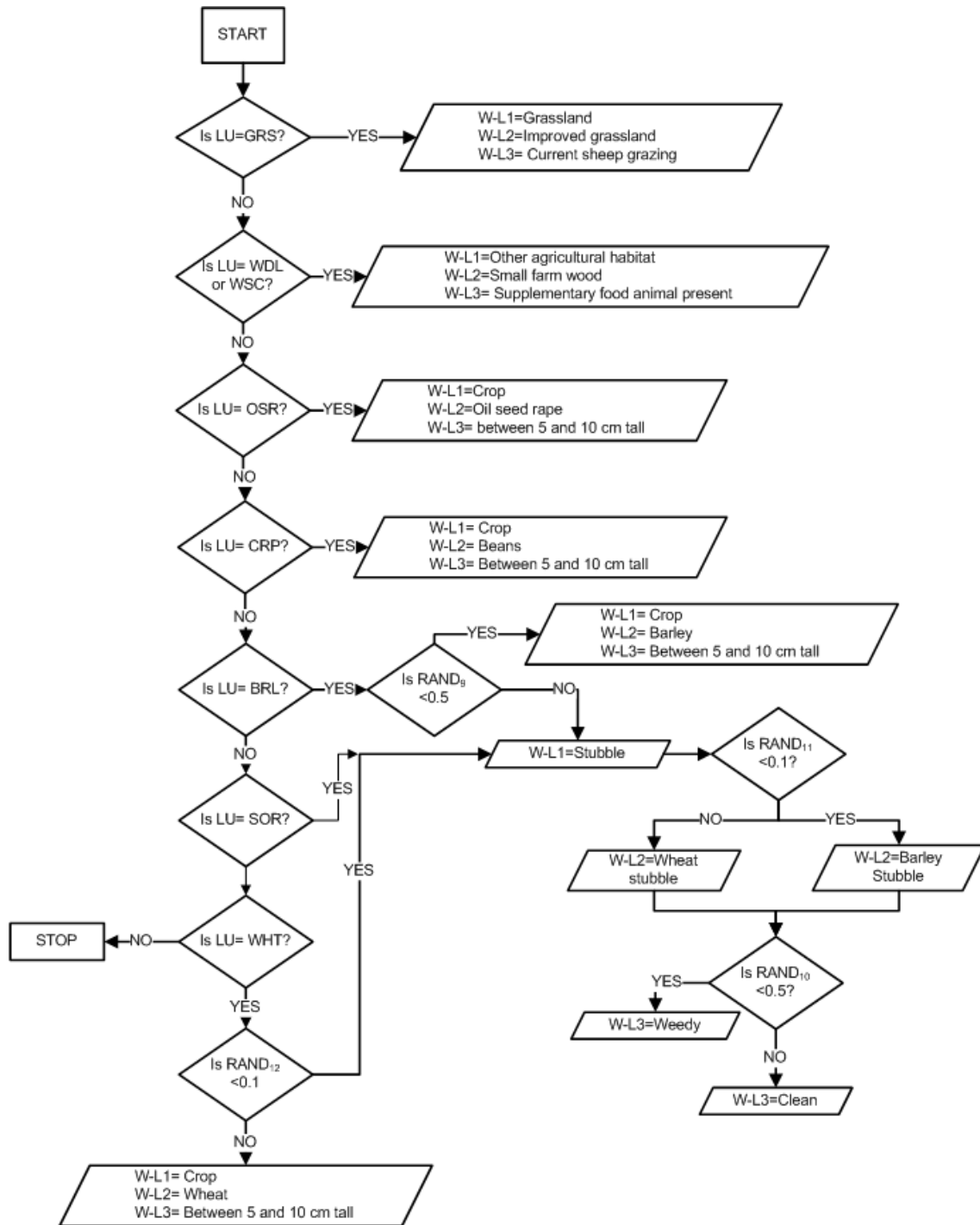
Fig. A.4. Winter habitat allocation algorithm applied. GRS, WDL, WSC, OSR, CRP, BRL, WHT are the land use (LU) classes as coded in Table 1; RAND() is a randomly generated number between 0 and 1, with the associated subscript number identifying the tier within the three level hierarchical WFBS habitat code structure; W-L1, W-L2 and W-L3 represent the three winter habitat levels.
