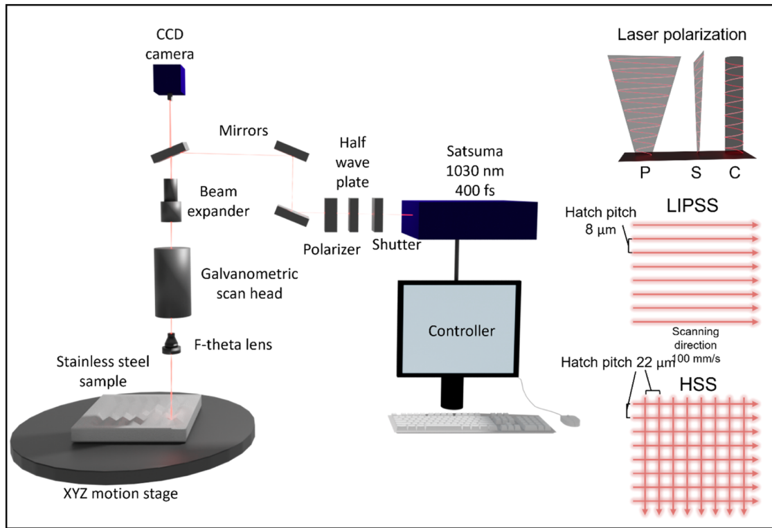
Fig. 3. Laser processing strategy used in this work.
