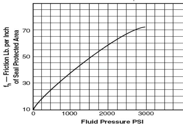
Figure 5: Friction due to Hydraulic Fluid Pressure 7
