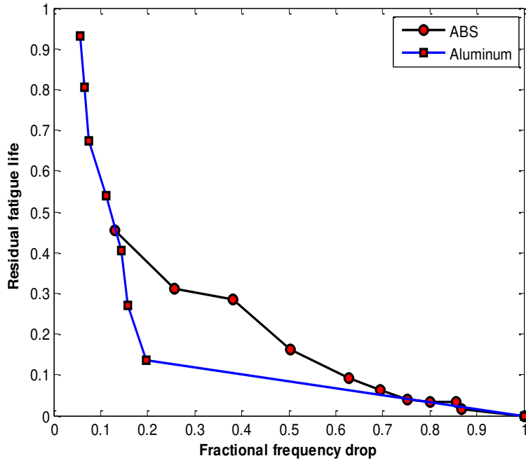
Figure 14: Residual fatigue life for a specimen having L = 130\text{mm}
