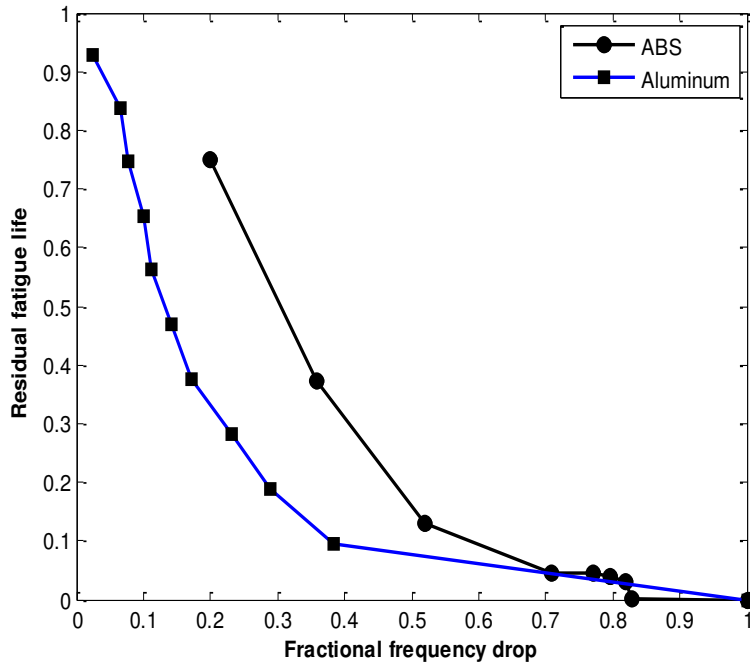
Figure 15: Residual fatigue life for a specimen having L = 150\text{mm}
