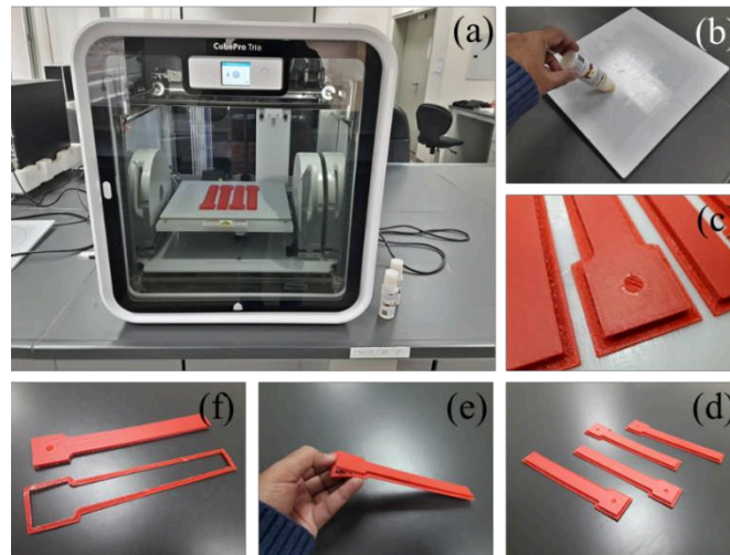
Figure 2: (a) CubePro Printer (b) applying glue on the platform (c) close view of the printed specimens (d) specimens after removal from the platform (e) removal of sidewalk and (f) ready specimen
