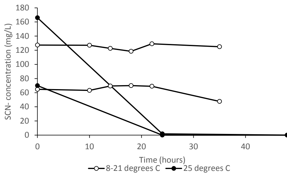
Fig. 3. Impact of temperature on \text{SCN}^- degradation in mixed culture batch tests. Thiocyanate degradation decreases when temperatures are sub-mesophilic.
