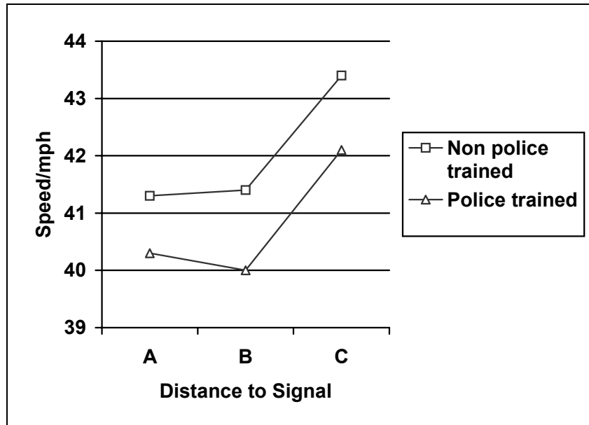
Figure 4: Mean Speed and Distance by Driver group (Traffic Lights)
