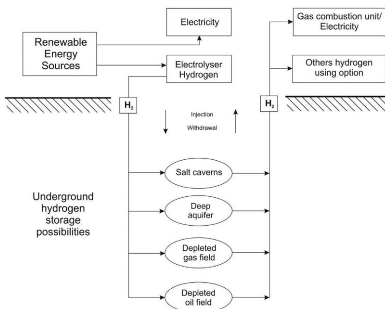
Fig. 2. underground hydrogen storage facility [25]
