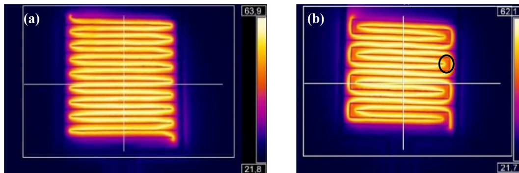
Fig. 8. (a) Thermograph image at 24 V of ECI 8001 ink (self-limiting T 65 °C) with 4COMB configuration and (b) 4SNAKE configuration where one of the areas showing temperature gradient within the heating area is highlighted in black.
