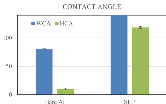
Fig. 5. Contact Angle results for water and Hexadecane on Bare Al (left) and SHP (right).
