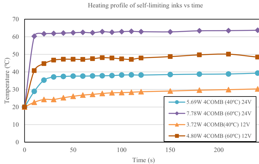
Fig. 9. Heating profile of the 4COMB configuration for the two self-limiting PTC inks at 12 V and 24 V.
