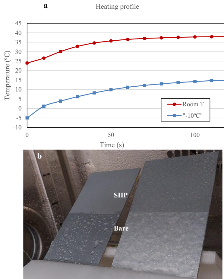
Fig. 10. (a) Heating profile of aluminum prototype at room temperature and at -10^{\circ}\text{C} ; (b) Image of reference sample and the hybrid prototype on the left side.
