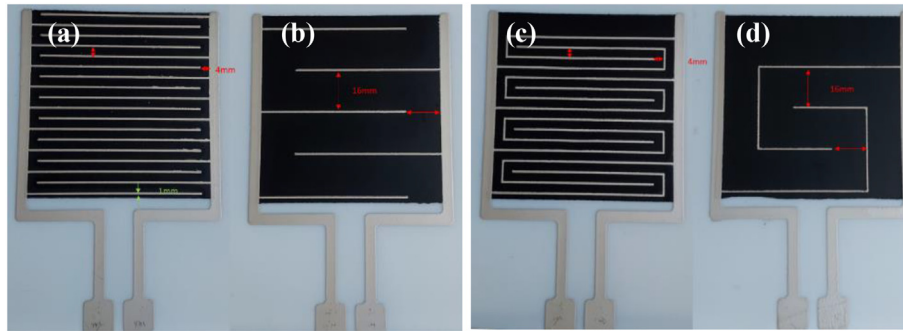
Fig. 6. Different configurations of Heater (a) 4COMB (b) 16COMB (c) 4SNAKE and (d) 16SNAKE.
