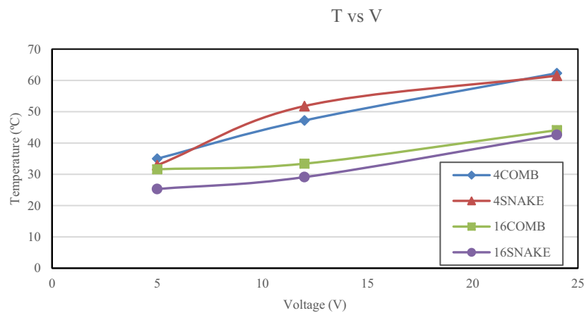
Fig. 7. Temperature of the different configurations under different voltages.
