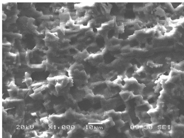
Fig. 4. SEM image of SHP surface.
