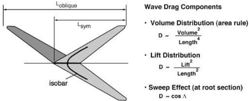
Fig. 33. Oblique wing drag reduction features (Source: [69])
