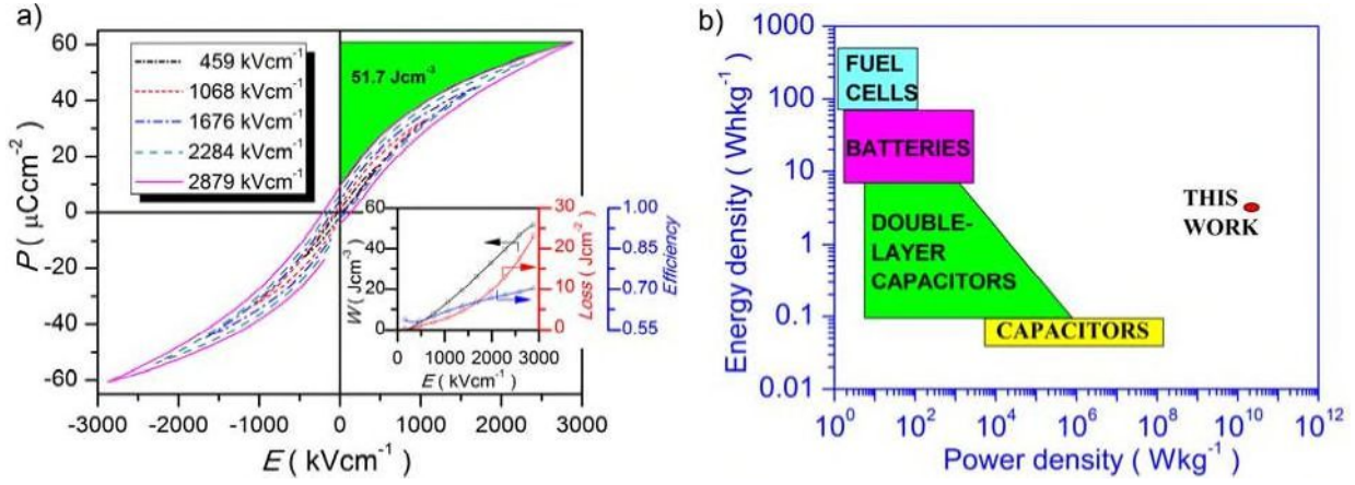
Figure 5. | Energy density and power density measurements of the BCT-BMT thin film. (a) P - E loops.
