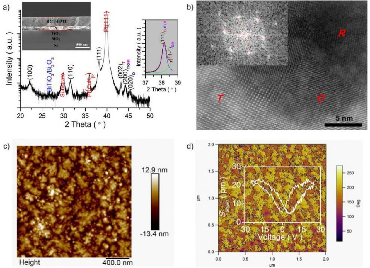
Figure 1. | 0.5(Ba 0.8 Ca 0.2 )TiO 3 -0.5Bi(Mg 0.5 Ti 0.5 )O 3 (BCT-BMT) thin film. (a) XRD pattern (diffraction intensity is in a logarithmic scale). A tiny amount (less than 1%) of secondary phases (BiTiO 3 or Bi 2 O 3 ) can be detected. Inset: cross-sectional SEM image. (b) Atom-scale HRTEM image. Inset: the fast Fourier transform spectrum of the R region. (c) Surface AFM micrograph. The average surface roughness of R a and R q is about 3.54 and 4.32 nm, respectively. (d) PFM vertical phase image. Inset: butterfly curve of the amplitude & voltage.
