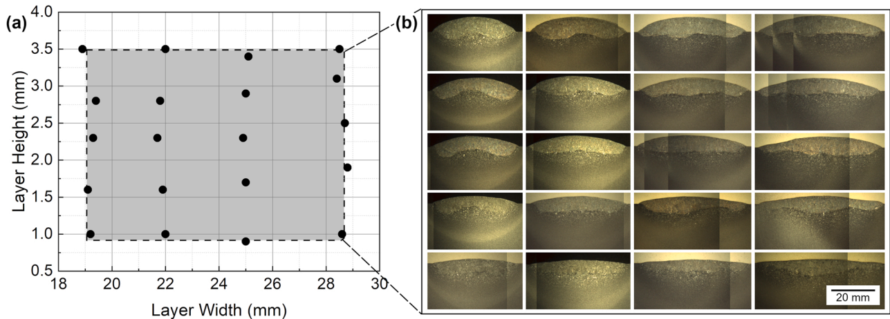
Fig. 17. (a) Scatter chart of layer height vs layer width correlation and (b) cross-section images.
