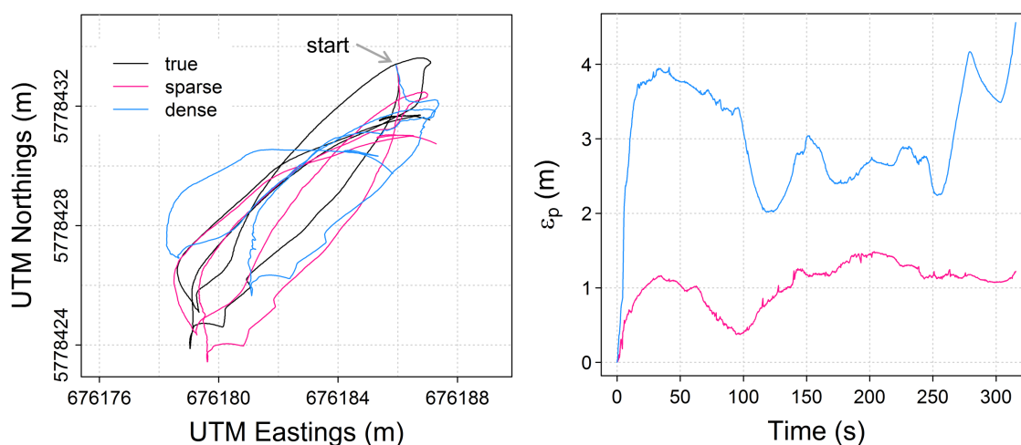
Figure 6. Position estimates (Left) and accumulation of 3D position error \varepsilon_p (Right) for a discharge measurement track of four consecutive river crossings.
