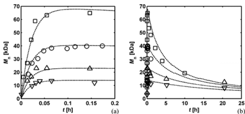
Fig. 15. Number average weight ( M_n ) for ROP of LA with \text{Sn}(\text{Oct})_2 and 1-dodecanol at 180^\circ\text{C} , [M]_0/[C]_0=10000 and [OH]_0/[C]_0=20 \square 34, \circ 60, \triangle 100, \nabla experimental results in dots and simulated results with dashed lines
