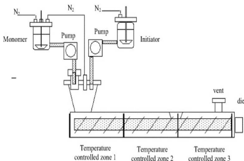
Fig. 11. Co-rotating twin-screw extruder for PCL polymerization
