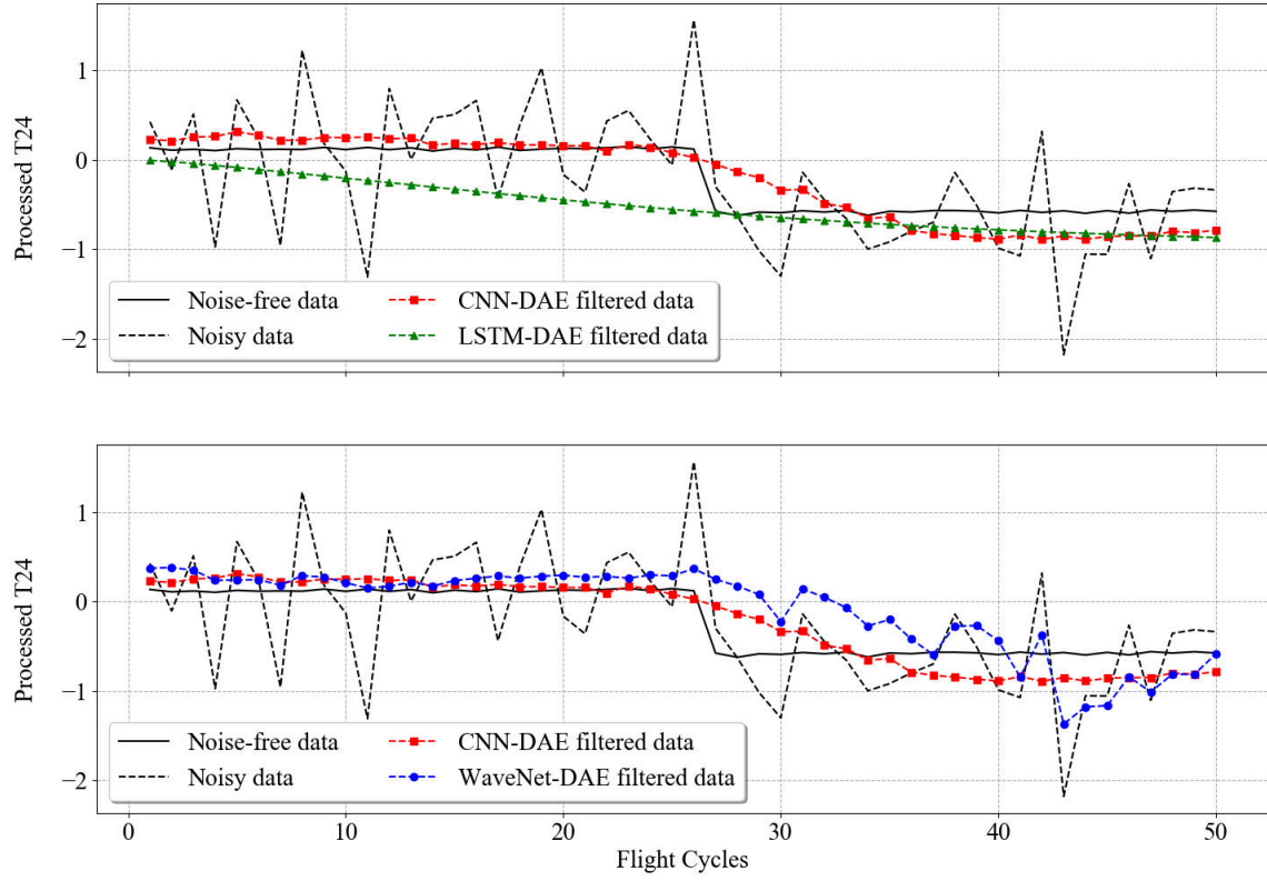
Fig. 12. Effect of LSTM-DAE and WaveNet-DAE ( -1.47\sigma T24 abrupt fault at flight 27).
