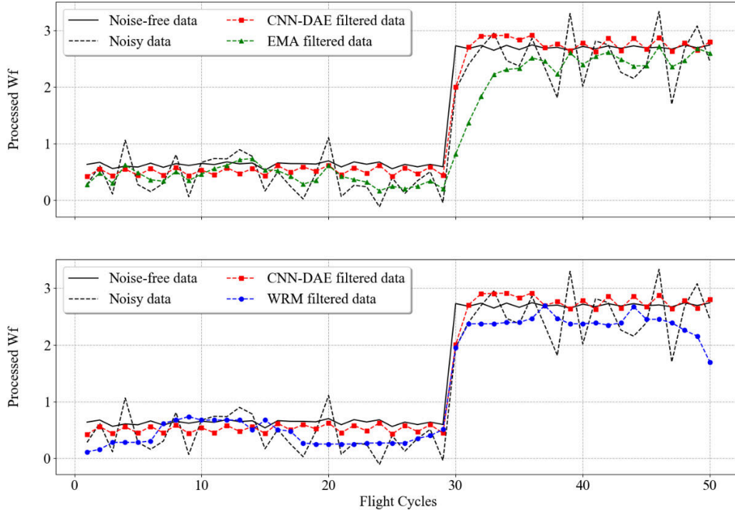
Fig. 10. Effect of EMA and WRM filters (8.16σ Wf sensor abrupt fault at flight 30).
