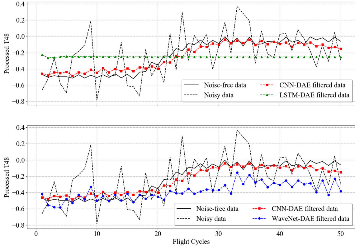
Fig. 13. Effect of LSTM-DAE and WaveNet-DAE ( 2.40\sigma T48 rapid fault at flight 17).
