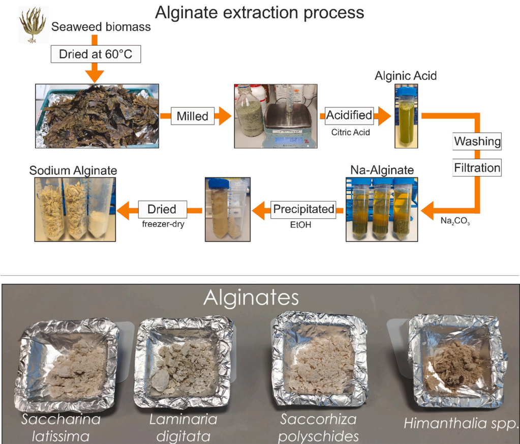
Fig. 2. Alginate extraction from Saccharina latissima , Laminaria digitata , Sacchorhiza polyschides , and Himanthalia spp.
