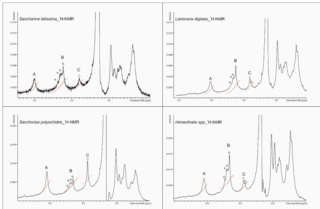
Fig. 3. ^1\text{H} -NMR spectrum (90 °C) of sodium alginate extracted from Saccharina latissima , Laminaria digitata , Sacchoriza polyschides , and Himanthalia spp. The ^1\text{H} -NMR spectra show specific peaks of the guluronic acid anomeric proton (G-1) peak A, mannuronic acid anomeric proton (M-1) peak B, and guluronic acid H-5 (G-5) and the C-5 of alternating blocks (GM-5) peak C.
