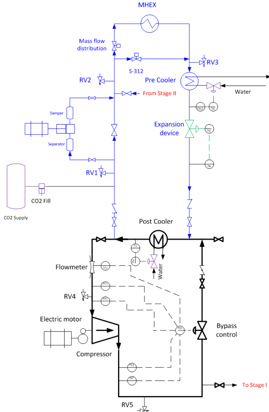
Figure 1 – Schematic of the envisaged S-CO 2 test rig. Blue: Stage I loop, Black: Stage II loop.
