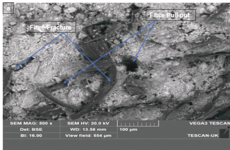
Figure 15a. SEM morphology of specimen reinforced with kraft and 2 wt.% banana fibre.
