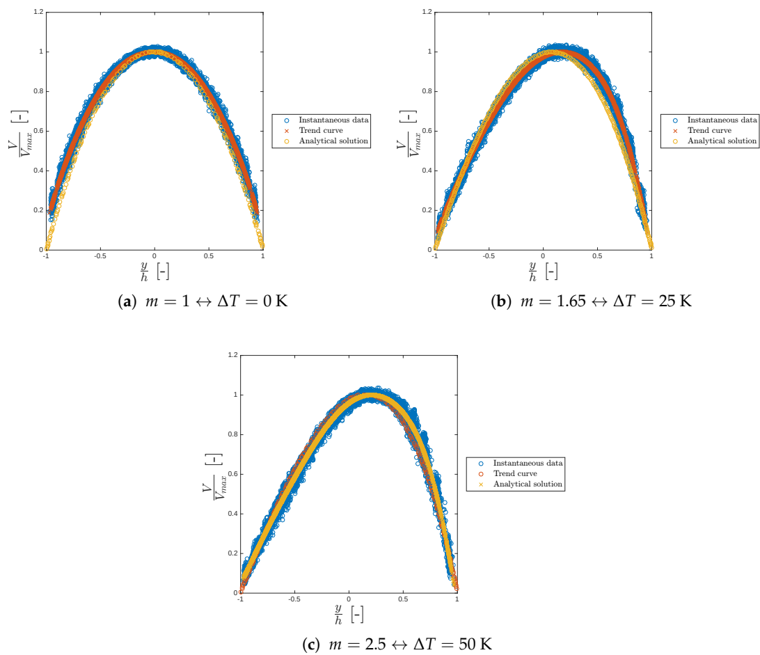
Figure 10. Dimensionless velocity profile for different m = \mu_{cold}/\mu_{ref} . Blue circles are the instantaneous data in the x direction, the orange curve is the trend curve extrapolated from the instantaneous data, yellow circles are obtained from the analytical solution from Sameen and Govindarajan [59].
