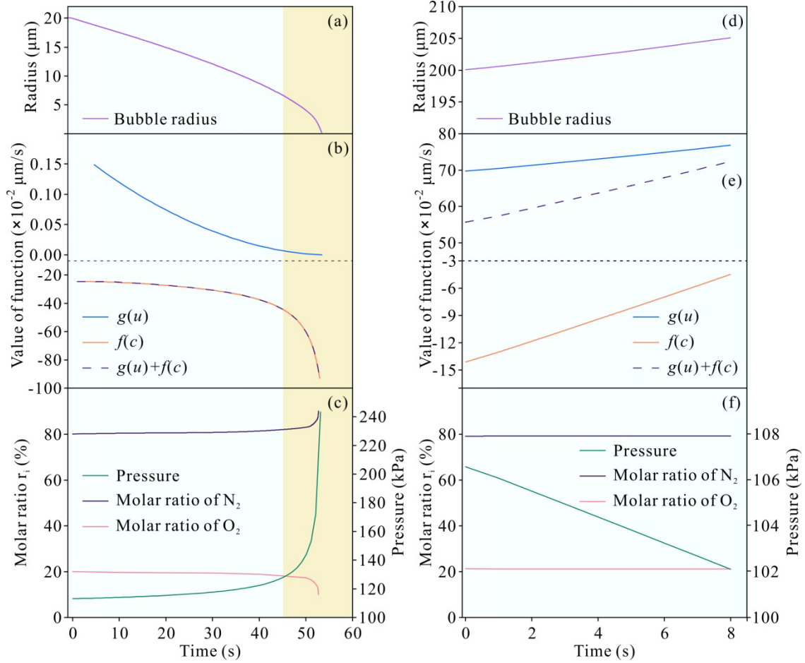
Fig. 3. Changes in bubble radius, the values of functions described by Eq. (20) and Eq. (21), the molar ratios of different gas components ( \text{N}_2 and \text{O}_2 ) and the inner pressure of the bubble. (a)-(c): the small bubble with an initial radius of 20 \mu\text{m} . (d)-(f): the big bubble with an initial radius of 200 \mu\text{m} . The water depths for all scenarios are 0.5 m.
