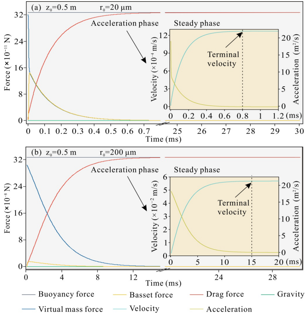
Fig. 2. The hydrodynamic forces and bubble motion characteristics (velocity and acceleration) during rising process for air bubbles at initial water depth of 0.50 m. Two initial radiuses of the bubble were considered at 20 \mu\text{m} (a) and 200 \mu\text{m} (b).
