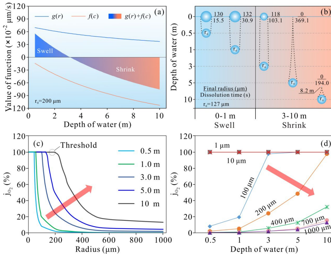
Fig. 6. (a) The shrink and swell potential for a 200 \mu\text{m} bubble at different initial water depths (0.5-10 m). (b) The final radius and position, and dissolution time for a 127 \mu\text{m} bubble at different initial water depths (0.5-10 m). (c) and (d) The oxygen utilization coefficient \dot{J}_{O_2} for bubbles with different initial radii (1-1000 \mu\text{m} ) at different initial water depths (0.5-10 m).
