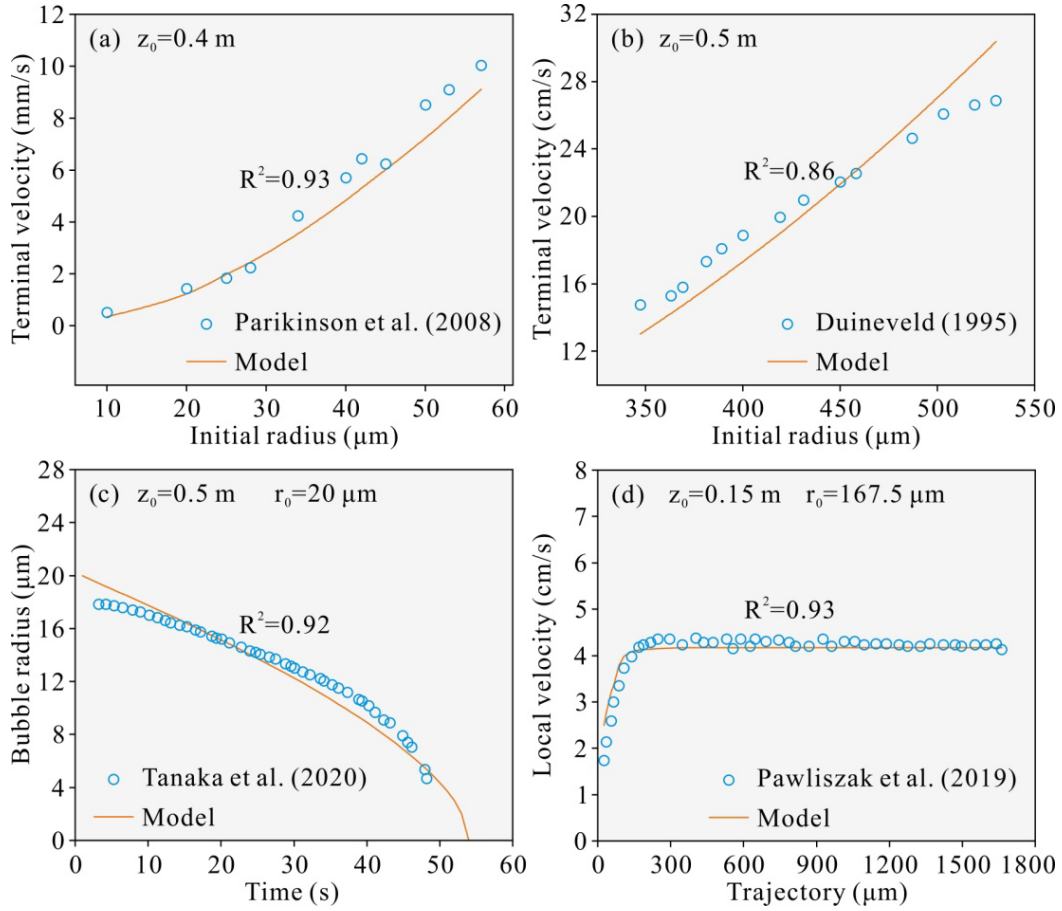
Fig. 4. Comparisons between experimental data and modelling results. Terminal velocity of bubbles with different initial radius 10-60 \mu\text{m} (a) and 350-530 \mu\text{m} (b); (c) Change of bubble radius during rising process, therein water depth is 0.5 m and initial radius is 20 \mu\text{m} ; (d) Bubble trajectory and local velocity, therein the initial water depth is 0.15 m and the initial radius is 167.5 \mu\text{m} . Terminal velocity denotes the velocity at the final stage of bubble rising, at this moment the variation of rising velocity in 1 s is less than 1%.
