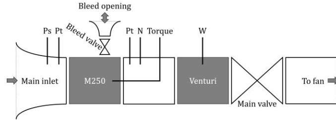
Fig. 9 Schematic illustration of sub-idle compressor bleed rig with its instrumentation.
