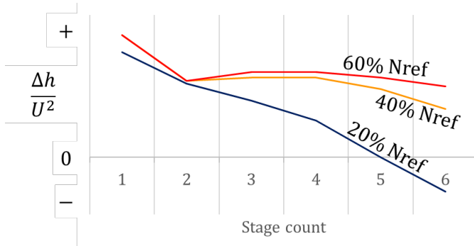
Fig. 2 Changes in stage matching for a 6-stage axial flow compressor analytical model during sub-idle (20% speed) and idle and above idle (40% and 60% speeds). The thermodynamic state of the flow entering a bleed near design when the corresponding stage is compressing may differ significantly from that during sub-idle when the stage could well be expanding (stages 5 and 6).
