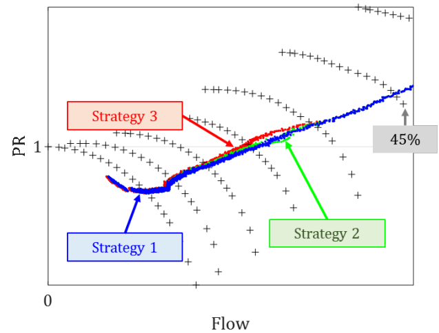
Fig. 17 Operating lines during a ground start (sub-idle region). Three operating lines are displayed: blue for strategy 1, green for strategy 2 and red for strategy 3. A map is shown in the background just for reference, note that each operating line uses several and different maps based on the bleed setting and the strategy followed.
