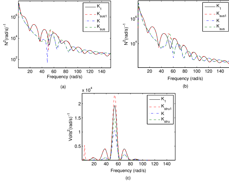
Figure 14: PSDs of control inputs: (a) left control force for active suspension (b) right control force for active suspension (c) control inputs for structural damping
