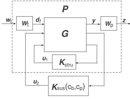
Figure 9: Design framework of controller
