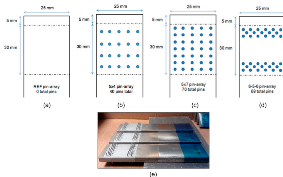
Figure 14. Schematics of micro-pin array patterns used in the experimental study: (a) no pins (Ref.), (b) 5 \times 4 pin array, (c) 5 \times 7 pin array, (d) 6-5-6 quincunx pin array, (e) the metal parts prior to joining with laminate in experiment.
