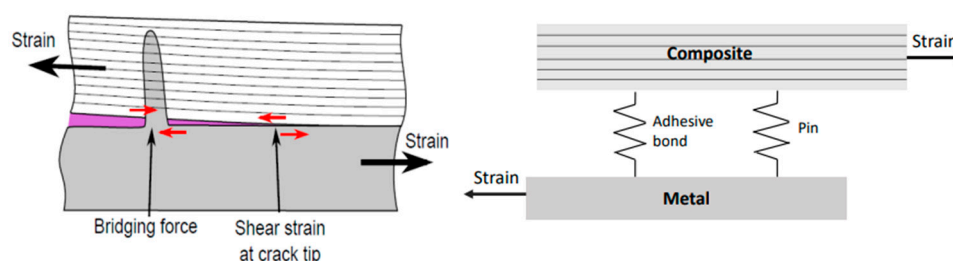
Figure 12. Schematic illustration of the effect of adherend axial stiffness on the effectiveness of pin traction in shielding the crack tip ( left ); the red arrows indicate the shear stresses. Insert figure ( right ) shows the two stress transfer elements: the pins and adhesive bond act like two springs working in parallel, transferring stress between the two adherends.
