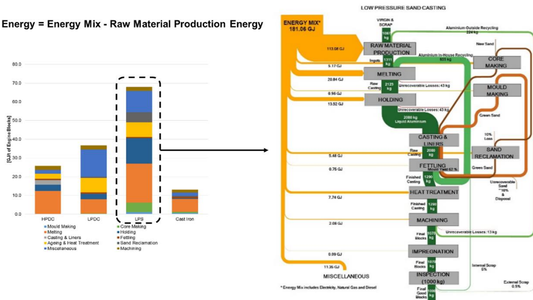
Figure 6: Sankey diagram showing energy and material flows for low pressure sand casting Al cylinder blocks
