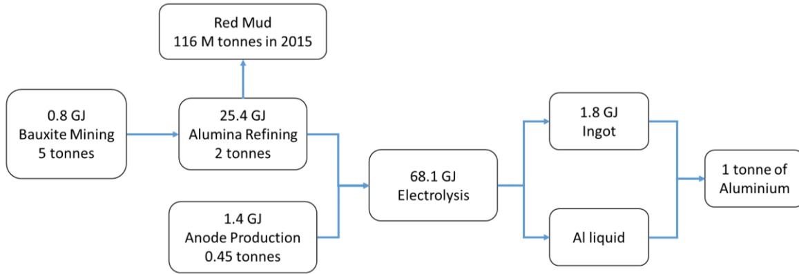
Figure 2: Process flow steps for primary aluminium production and corresponding energy content required to produce 1 tonne of aluminium
