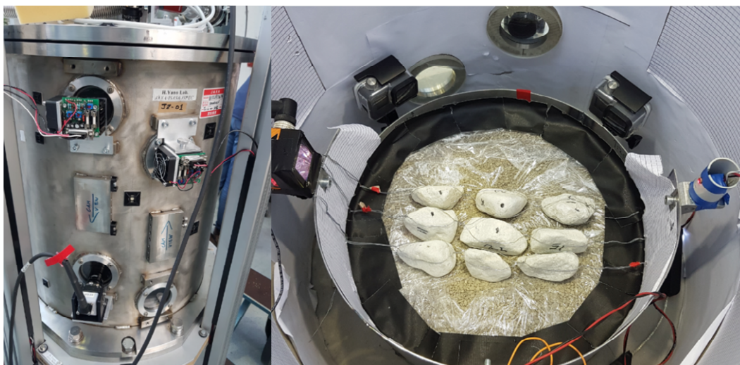
Figure 6. Sensors Setup. The external view (left) shows the bottom FC camera and two lamps attached to windows on the side of the vacuum chamber. The interior view (right) shows the two GoPros, separated by 90°, with the FC camera seen from the middle window. The light gate is seen attached at the top of the container, with the receptor (right side in blue) diametrically opposed to the emitter.
