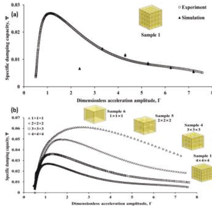
Figure 16. (a) Comparison of experimental with the simulation results at various acceleration values for a sample with 64-unit cubes inside and (b) SDC values of the samples at various acceleration values with varying sample cells inside for 1-, 8-, 27-, and 64-unit cubes inside (Reproduced with permission from. [18] Copyright 2022, Elsevier)
