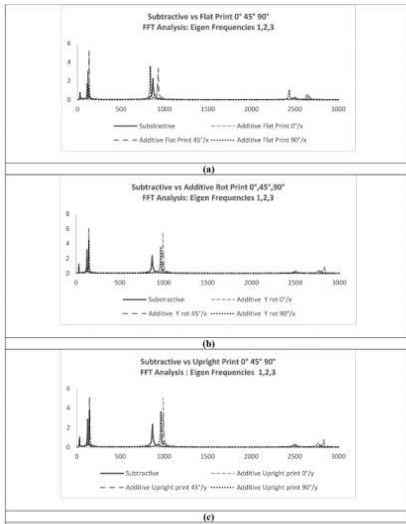
Figure 2. The Fast Fourier Transform (FFT) analysis observed for the subtractive and AM manufactured samples at 0°, 45°, and 90° for orientation of (a) Flat, (b) Rotation, and (c) Upright (Reproduced with permission from. [21] Copyright 2022, Elsevier)
