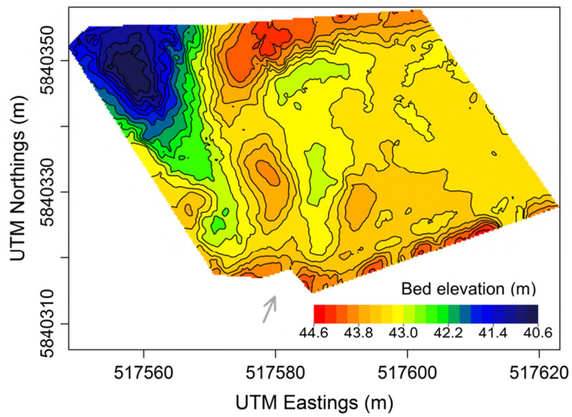
Figure 10. Bed elevation downstream of Shrewsbury weir; the elevation is referenced to the mean sea level as obtained from GPS; the grey arrow points to the location of the fish pass entrance and is orientated perpendicular to the front wall of the fish pass.
