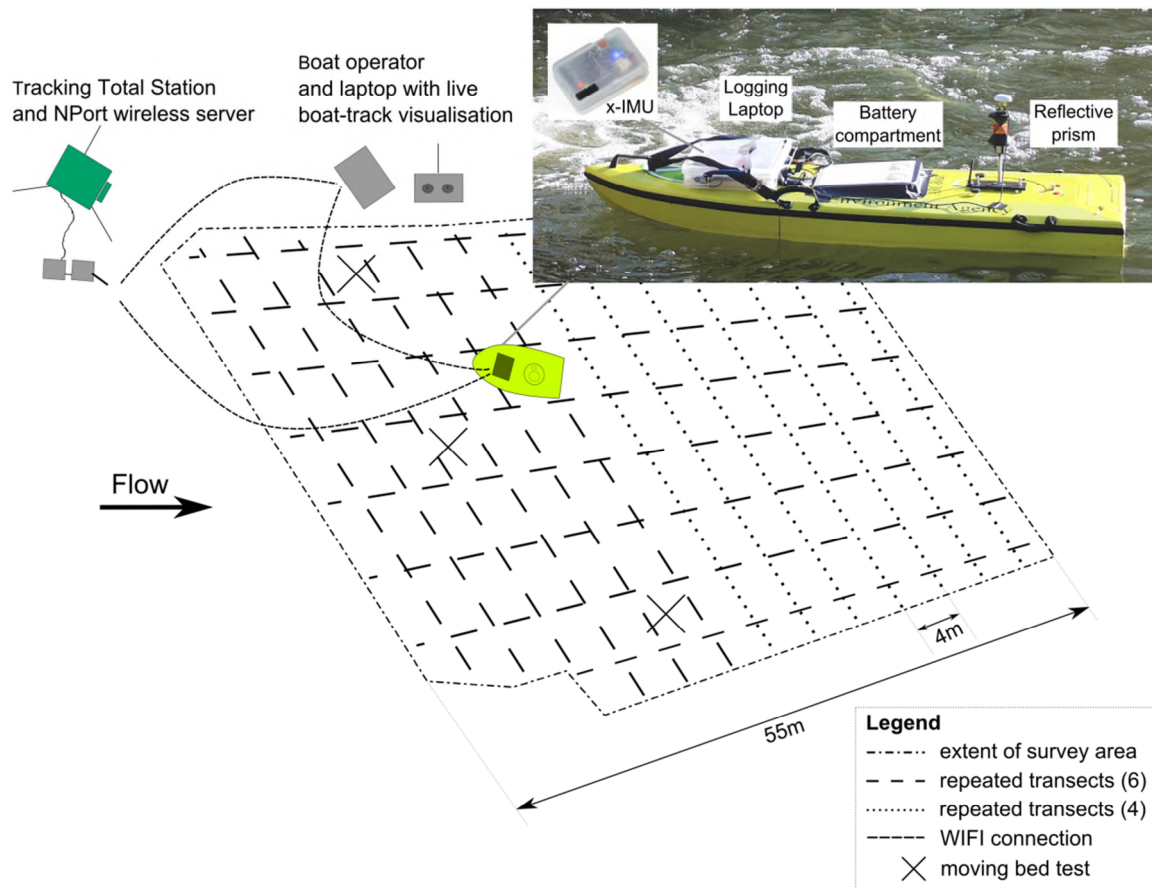
Figure 2. Sampling strategy and technical survey setup (not to scale).
