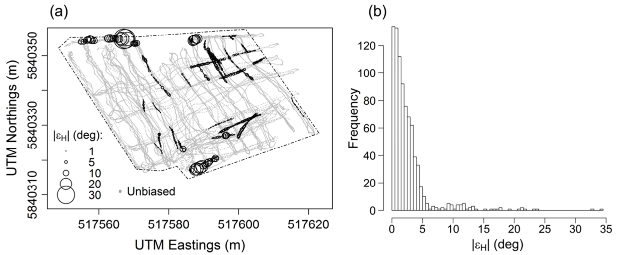
Figure 5. (a) Spatial distribution and magnitude of the detected absolute ADCP compass error ( |\epsilon_H| ); the dash-point line denotes the extent of the study area; (b) Statistical distribution of |\epsilon_H| (n=836).
