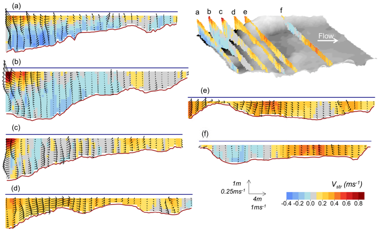
Figure 12. Spatial water velocity distribution at selected cross sections downstream of Shrewsbury Weir; the top right plot shows the location of the cross sections on a 3D bathymetric display (see also Figure 1) and plots (a) to (f) show the streamwise velocities ( V_{str} ) as well as the cross-stream and vertical velocities (depicted as arrows) of these sections in detail.
