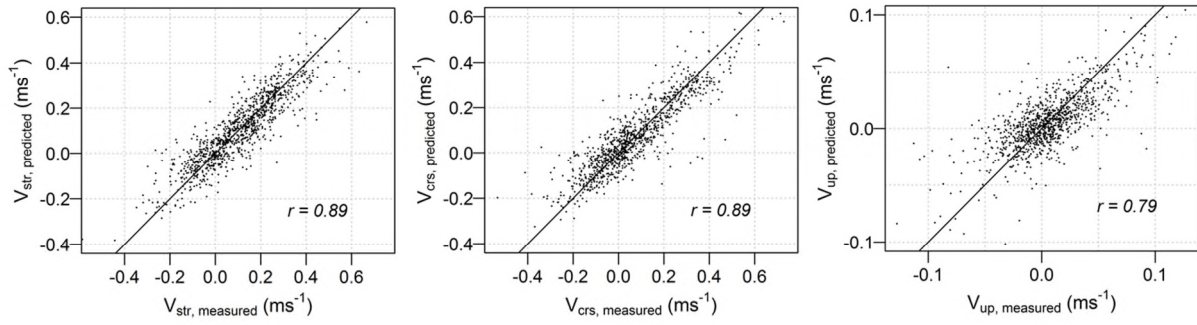
Figure 9. Cross-validation of spatial water velocity interpolation through ordinary kriging; str , crs , up and r stand for streamwise, cross-stream and vertical and for linear correlation coefficient, respectively. The diagonal line in each subplot denotes the slope of 1.
