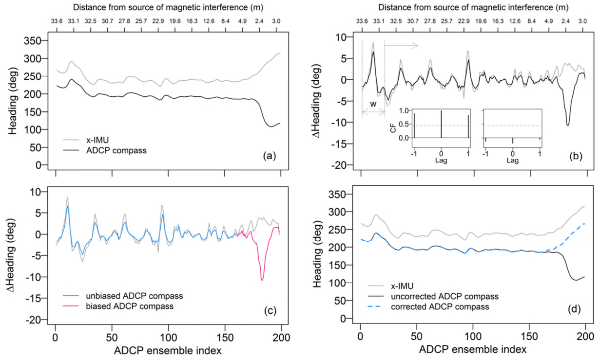
Figure 3. ADCP-IMU integration illustrated using data collected on a cross section of the River Thames at Eynsham, Oxfordshire (UK), with a moored steel hulled vessel acting as source of magnetic interference; (a) Time synchronised data of ADCP compass and x-IMU; (b) Detection of biased ADCP compass data; the two inlay plots show the results of the cross-correlation analysis for unbiased (left plot) and biased (right plot) compass data, where CF stands for cross-correlation function; (c) Results of the compass error detection; (d) Results of the compass error correction.
