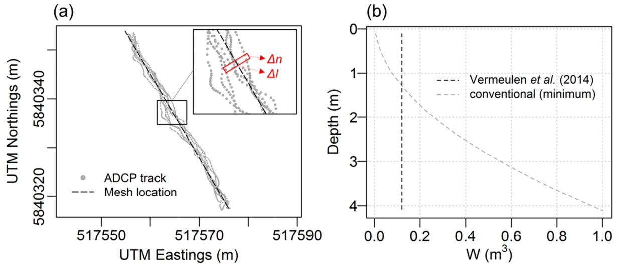
Figure 4. (a) Plane view of the 3D velocity projection mesh on the ADCP track (shown for section b in Figure 1); \Delta l and \Delta n stand for the longitudinal and the lateral mesh cell dimensions; (b) Volume ( W ) for which spatially homogeneous flow is assumed in the processing method by Vermeulen et al. (2014) with the cell dimensions used in this study and the minimum W in conventional processing of data from a 1200 kHz WorkHorse RioGrande ADCP with a vertical measurement resolution of 0.12m; an instrument draft of 0.11m was assumed for both methods.
