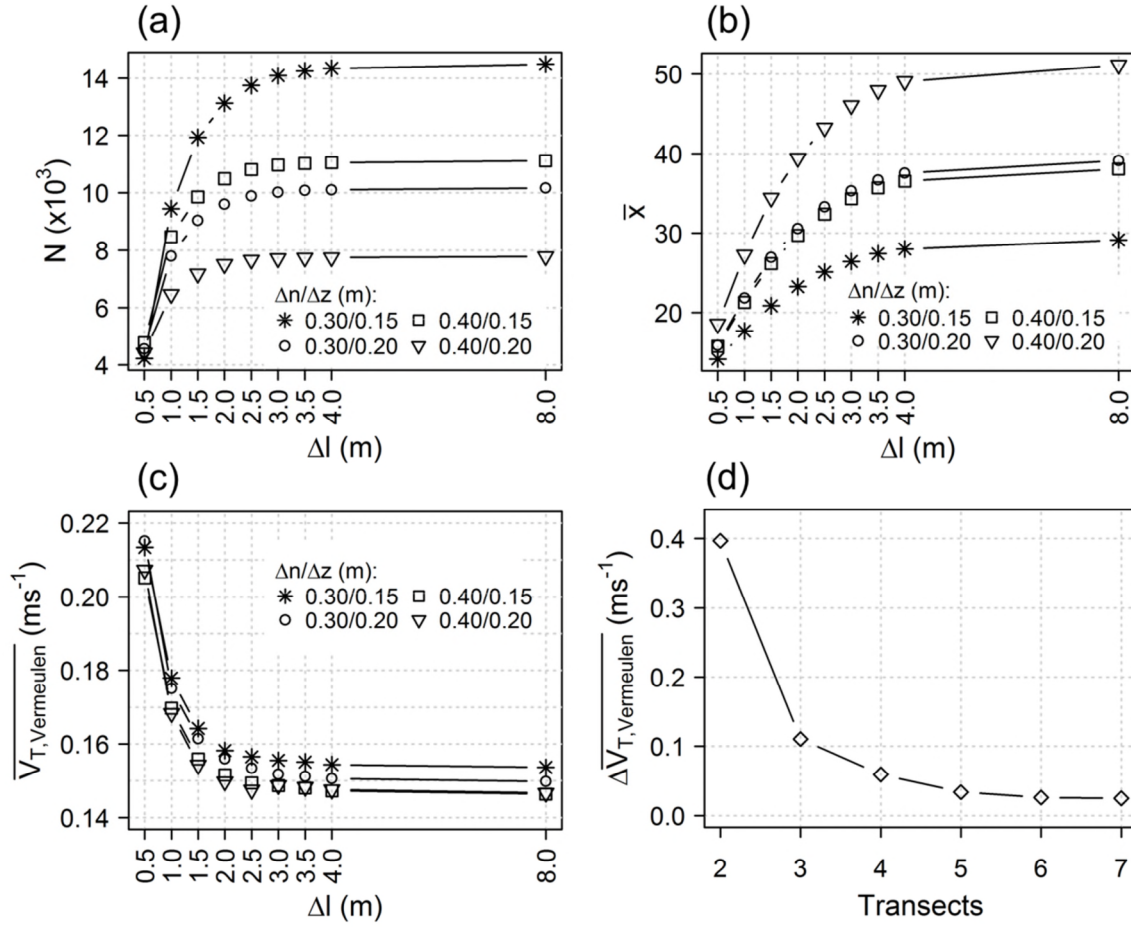
Figure 8. Sensitivity analysis for the 3D velocity estimation by Vermeulen et al. (2014); (a, b) Sensitivity of the total number of cells with 3D velocity estimates ( N ) and the average number of along-beam velocity samples per cell ( \bar{x} ) to the mesh cell dimensions (shown for the data of all sections processed); (c) Sensitivity of the estimated average water velocity magnitude in the mesh cells of a section ( \overline{V_{T,Vermeulen}} ) to the mesh cell dimensions (shown for the data of section b in Figure 1); (d) Change in the estimated average water velocity magnitude ( \Delta \overline{V_{T,Vermeulen}} ) caused by including another transect, calculated for mesh cell dimensions of \Delta l=2.00\text{m} , \Delta n=0.40\text{m} and \Delta z=0.15\text{m} (shown for the data of section b in Figure 1).
