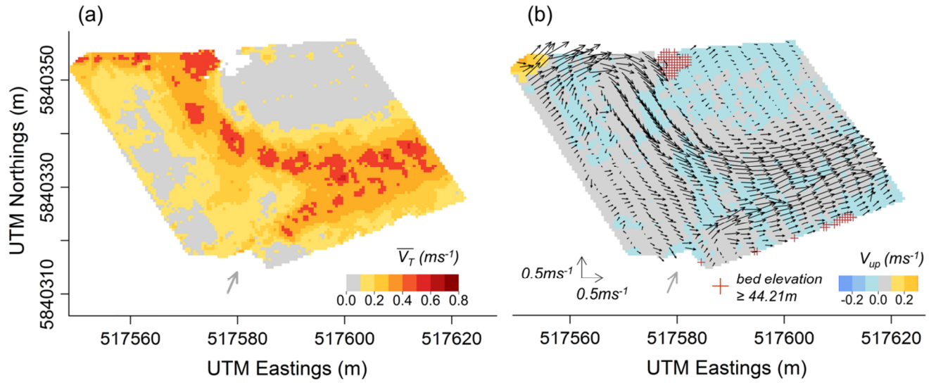
Figure 11. Spatial water velocity distribution downstream of Shrewsbury Weir; (a) Magnitude of depth-averaged velocities ( \overline{V_T} ); (b) Streamwise and cross-stream velocities (depicted as arrows) and vertical velocities ( V_{up} ) at an elevation of 44.21m above the sea level, corresponding to a distance of 0.35m below the mean water surface elevation of the study area; the grey arrow in both plots (a) and (b) points to the location of the fish pass entrance and is orientated perpendicular to the front wall of the fish pass.
