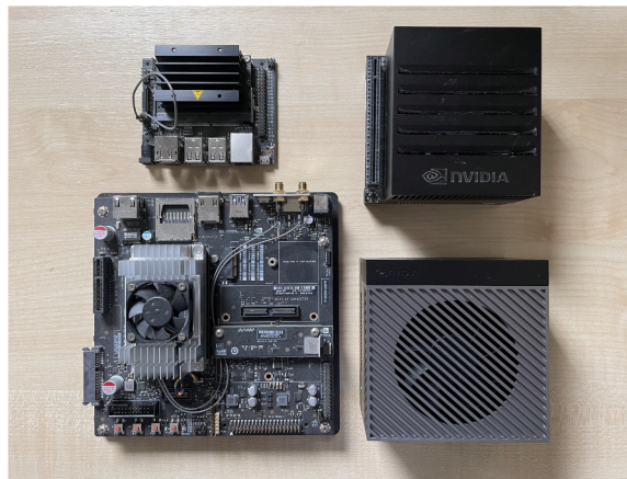
Fig. 3. Edge computing modules used in the latency test. Top eft: Jetson Nano. Top Right: Jetson AGX Xavier. Bottom left: Jetson TX2. Bottom right: Jetson AGX Orin.
