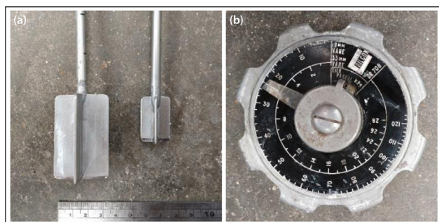
Figure 1. Shear vane test apparatus
