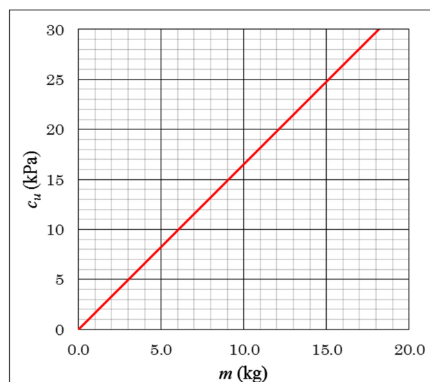
Figure 9. Design chart for strength of sludge at which penetrometer sinks under self-weight
