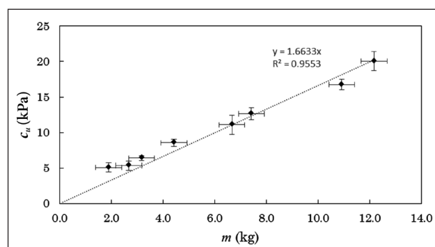
Figure 4. Static penetration test data
